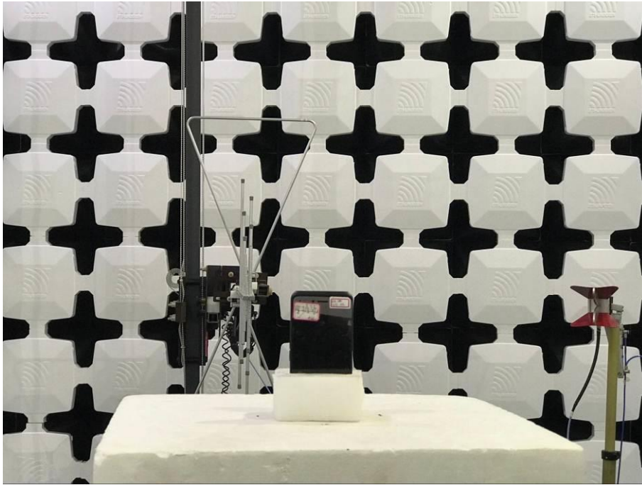
9. Radiated Emissions (Part 22/24) (Above 3GHz)
