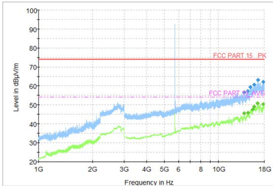
Fig. 102 Transmitter Spurious Emission (802. 11a 5785MHz)
