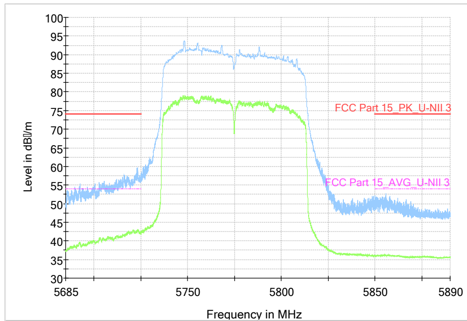
Fig. 62 Band Edges (802.11ac-VHT80, 5775MHz)
