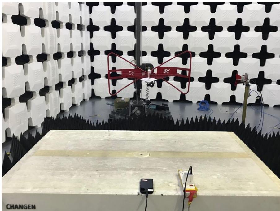
6. Radiated Emissions (Part 15B Camera/ Scanner/Video Player,1GHz-18GHz)
