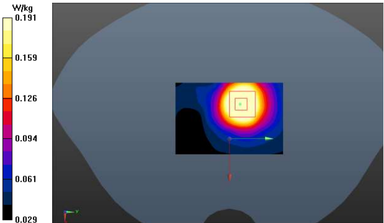
Fig.2 Bluetooth Body
