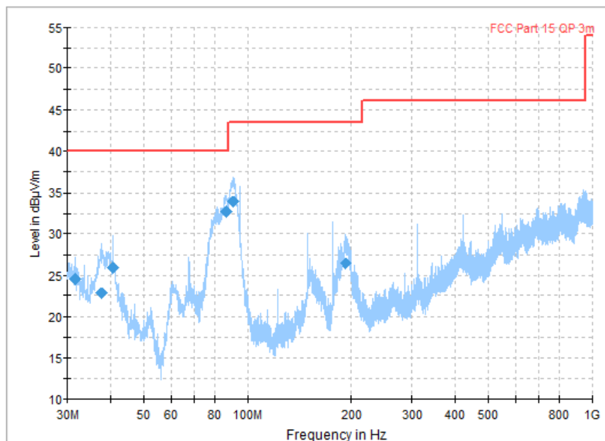
Figure A-3 Transmit State (30M-1G)
