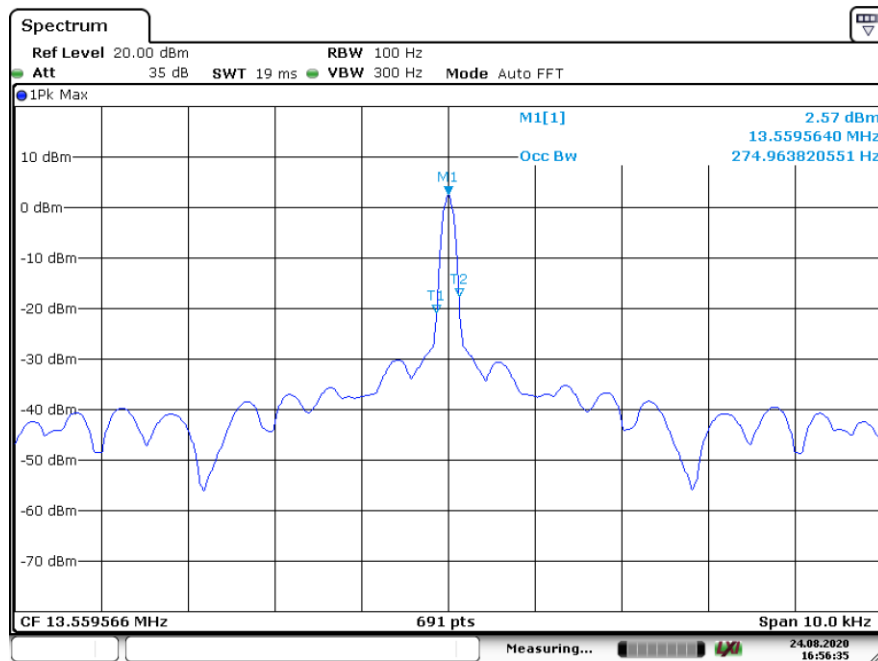
Figure A-6 Occupied Bandwidth
