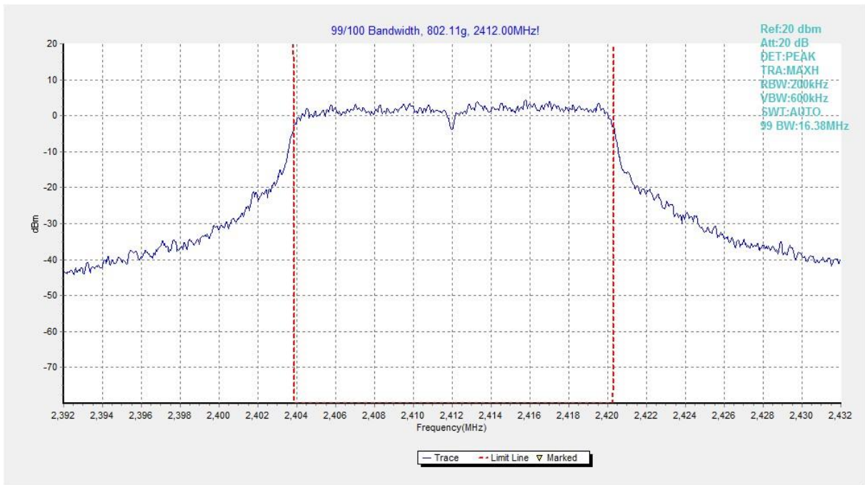
Fig.65 99% Occupied Bandwidth (802.11g, CH 1)
