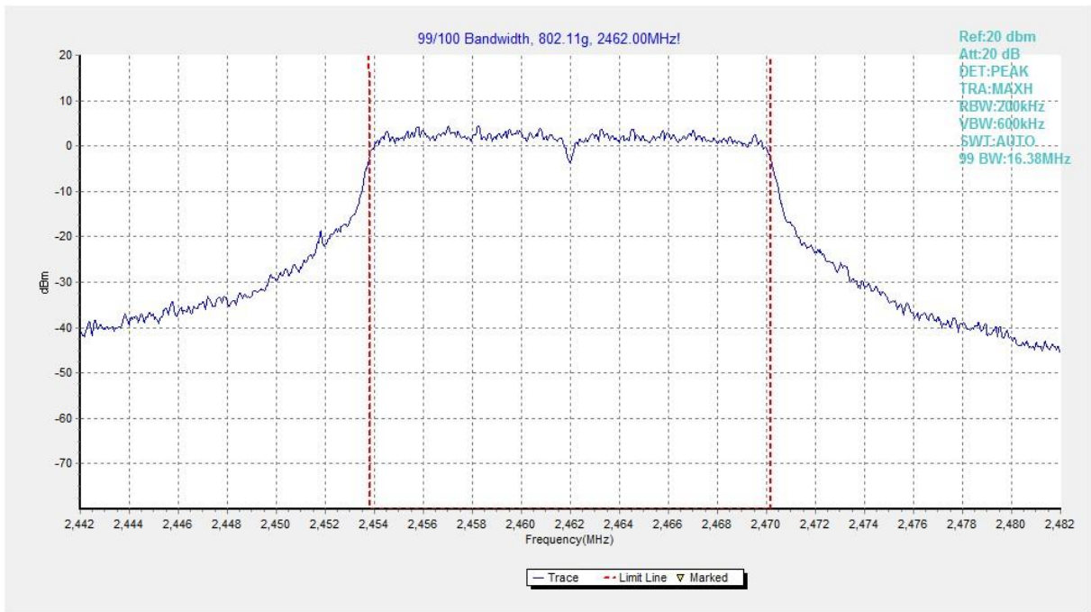
Fig.67 99% Occupied Bandwidth (802.11g, CH 11)
