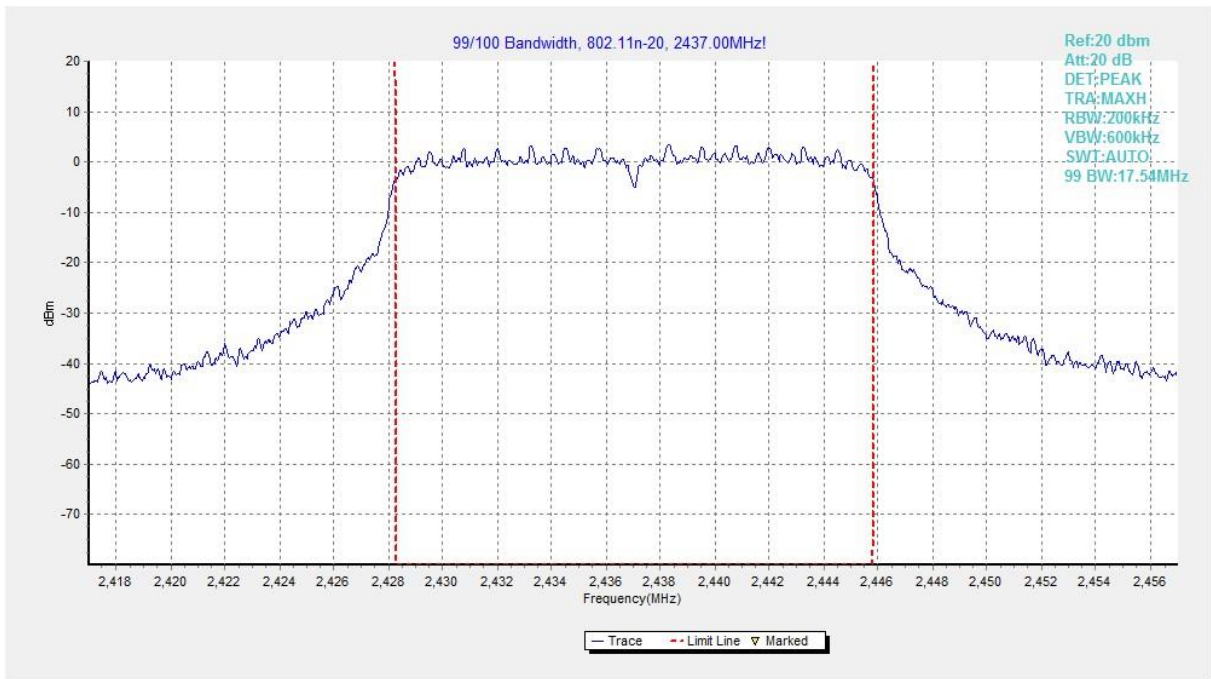
Fig.69 99% Occupied Bandwidth (802.11n HT20, CH 6)
