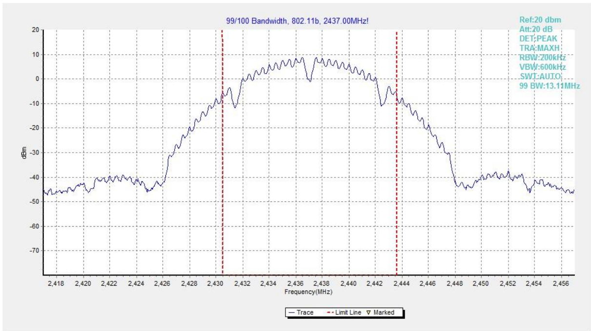
Fig.63 99% Occupied Bandwidth (802.11b, CH 6)
