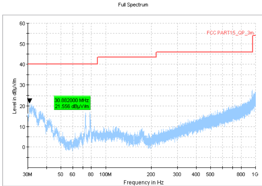
Fig.50 Radiated Spurious Emission (All Channels, 30MHz-1 GHz)
