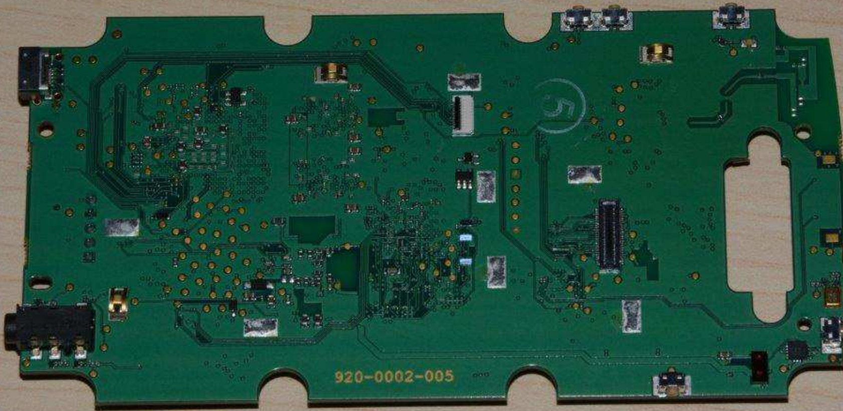
8741/8753 Main Board Front View
