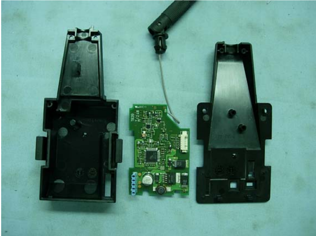
Internal View (Removed Covers, RF Board/Front View)
