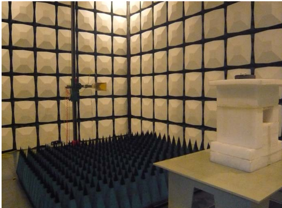
Radiated Emission View (Above 1GHz)
