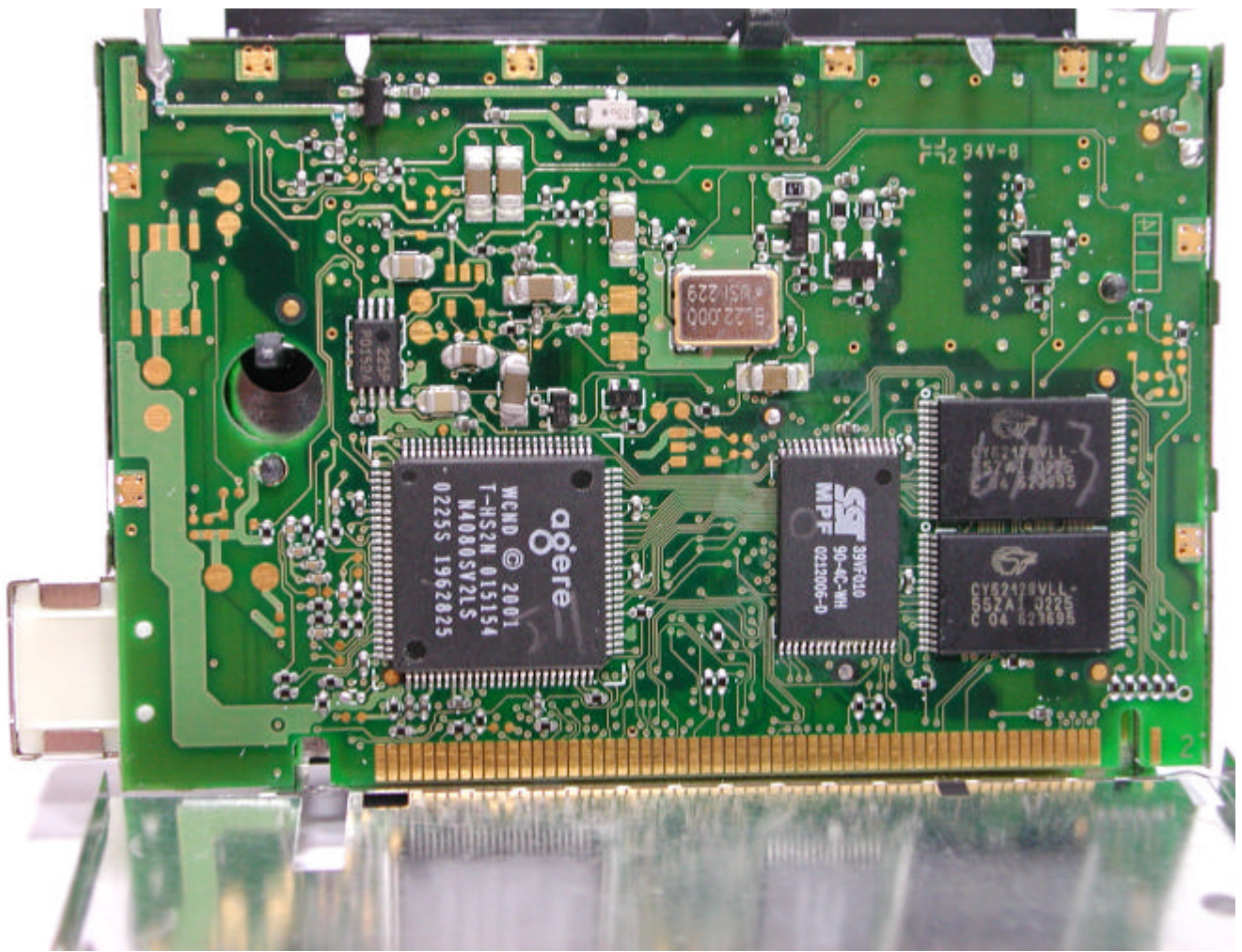
Interior Photo of the USI LC_USB
