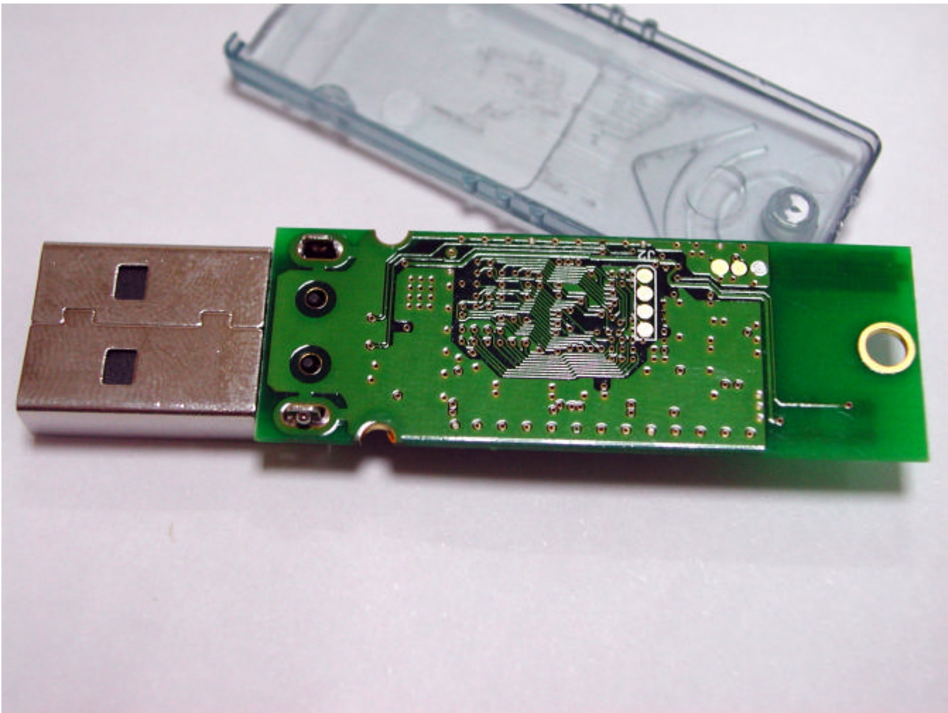
Internal Photo of the USI UD-23011
