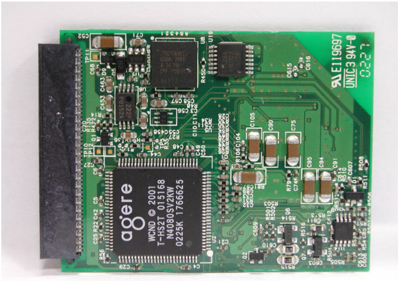
Internal Photo of USI 802.11b CompactFlash Card
