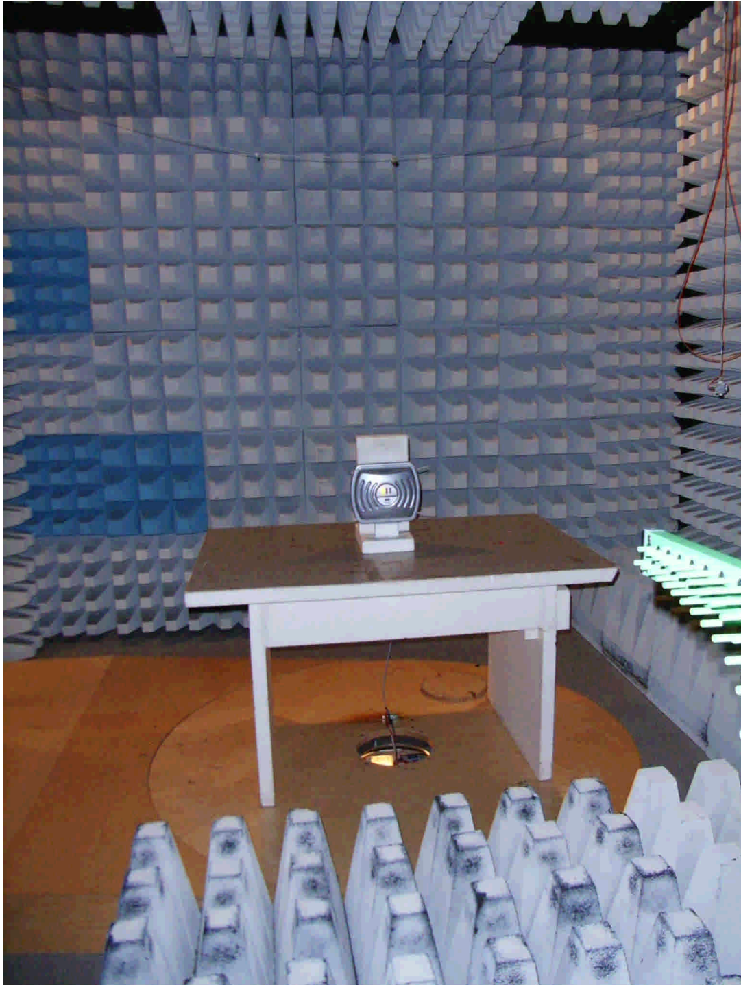
91187_16.jpg TSU25, test setup fully anechoic chamber
