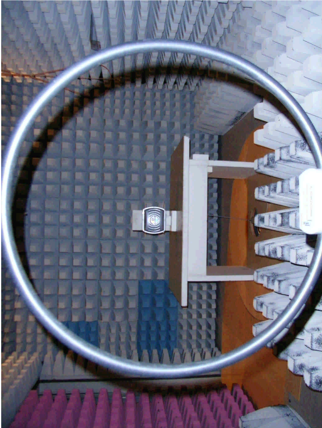
91187_23.jpg TSU25, test setup fully anechoic chamber
