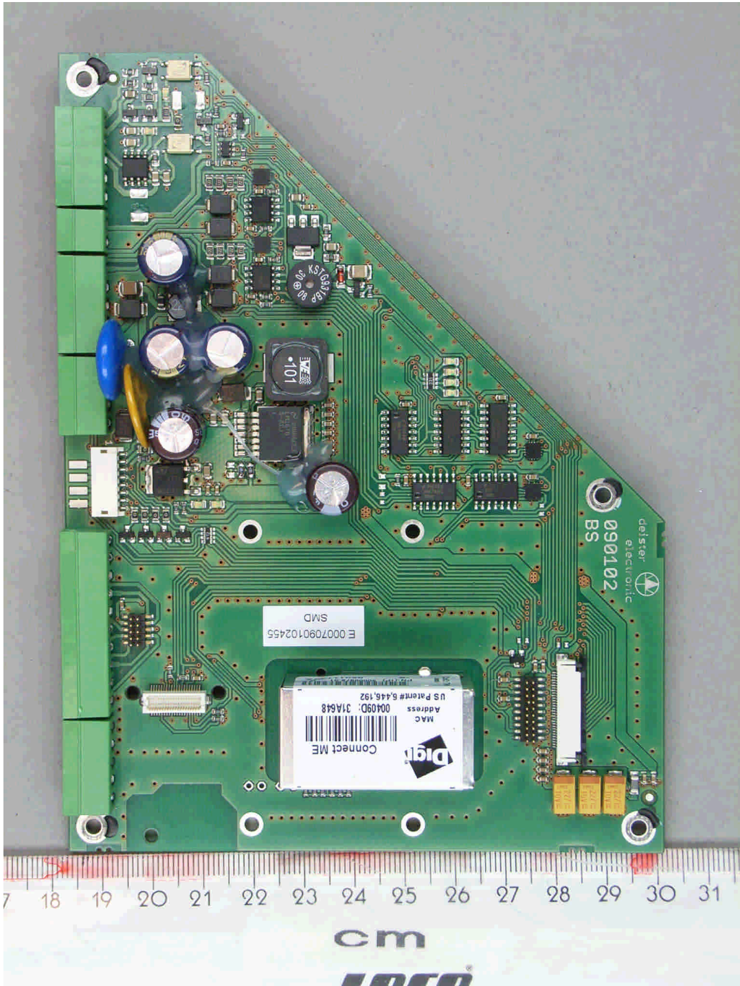
91187_k.jpg TSU25, main PCB, top view
