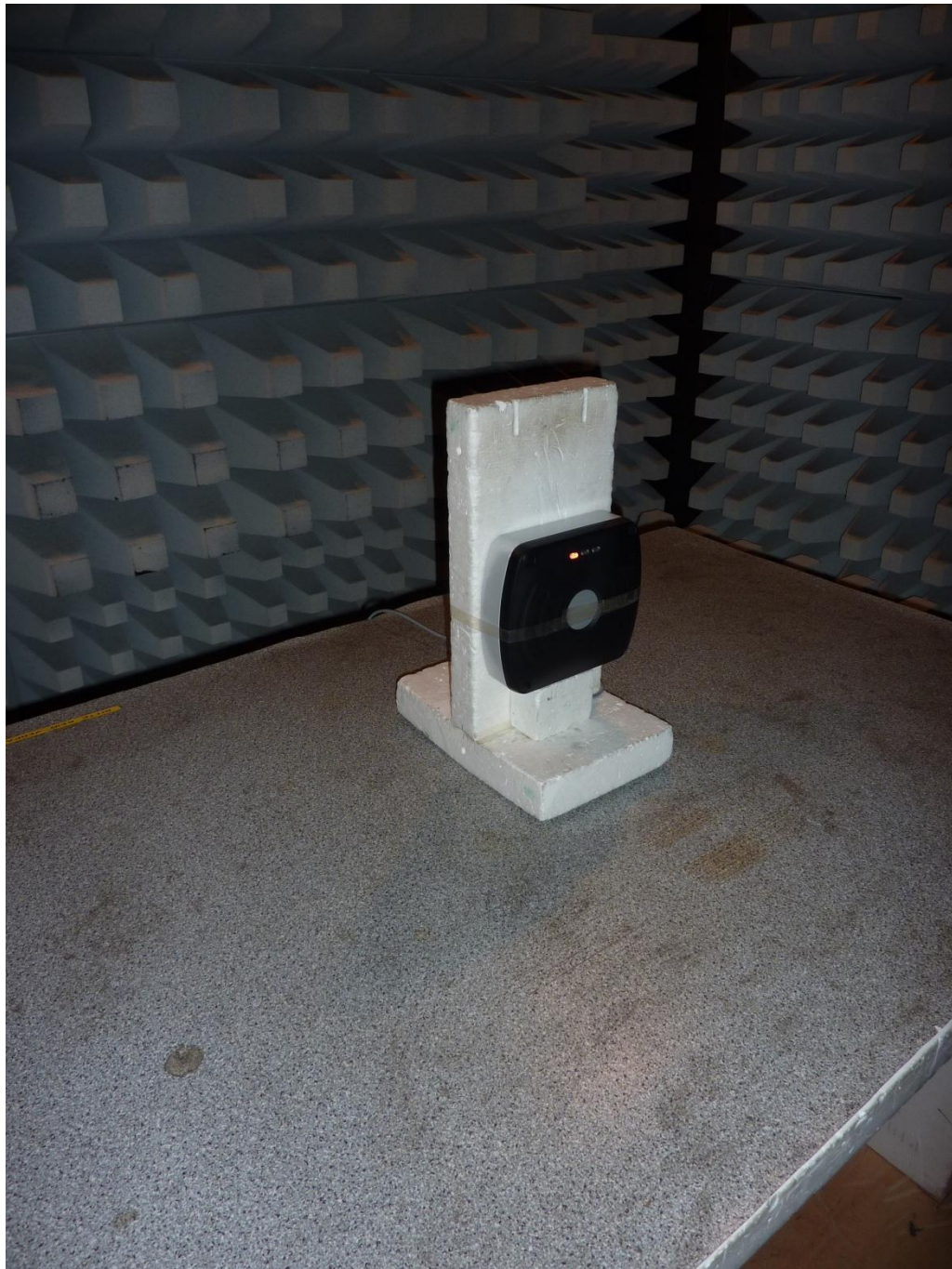
122887_16.JPG: TSU200, test set-up fully anechoic chamber
