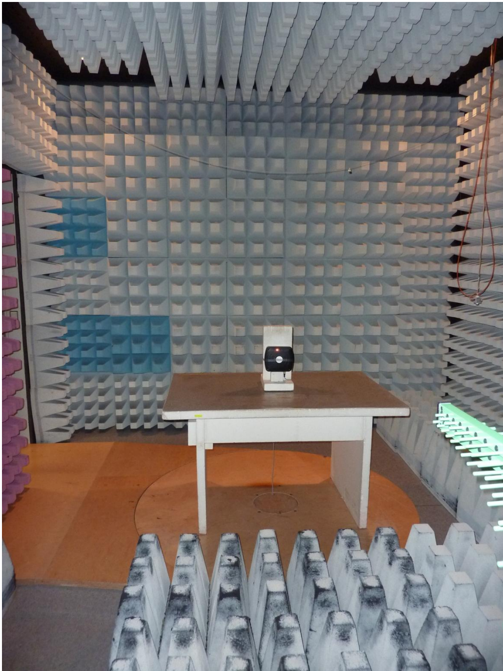
122887_21.JPG: TSU200, test set-up fully anechoic chamber
