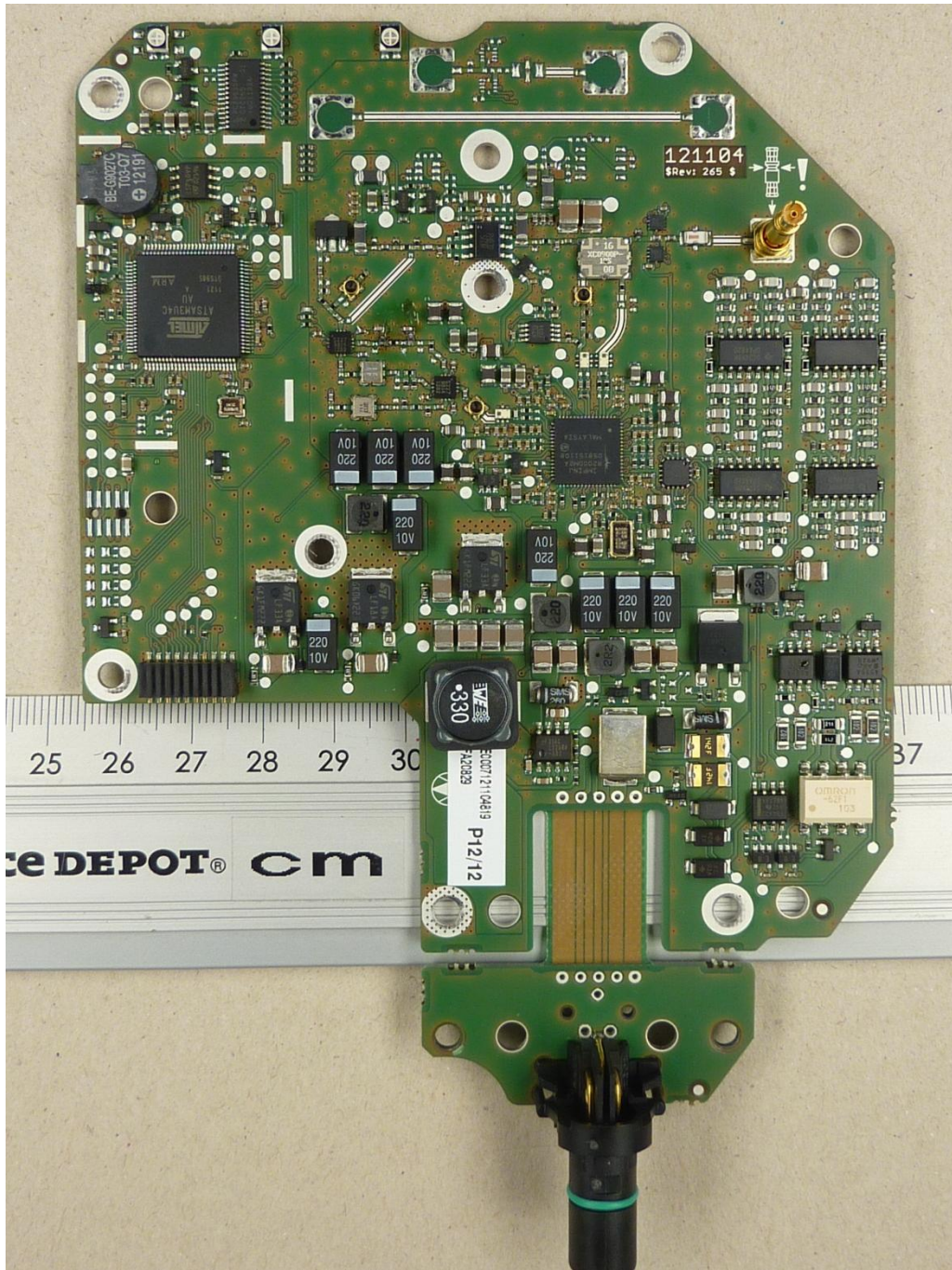
122887_q.JPG: TSU200, main PCB, top view
