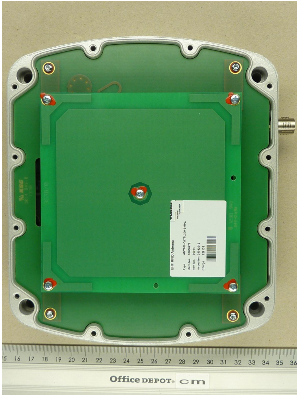
122887_o.JPG: TSU200, internal view 1 (cover removed)
