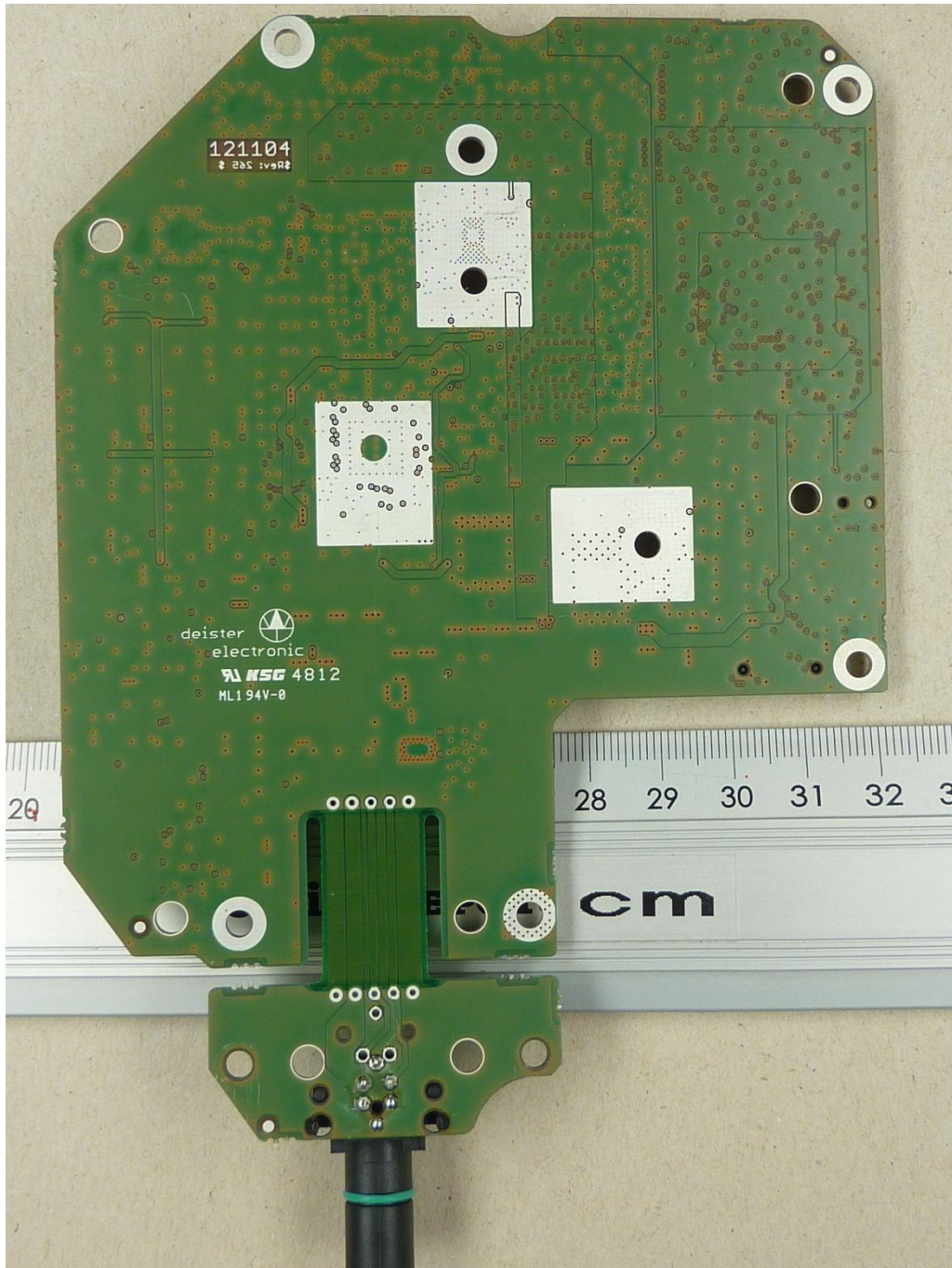
122887_r.JPG: TSU200, main PCB, bottom view
