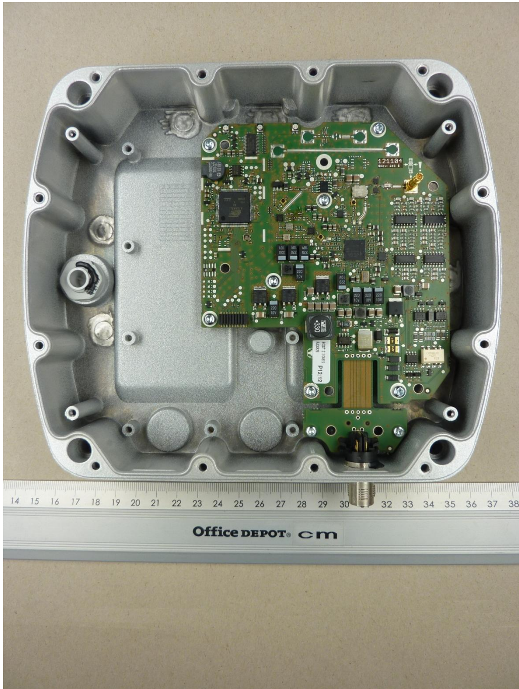
122887_p.JPG: TSU200, internal view 2 (antenna removed)
