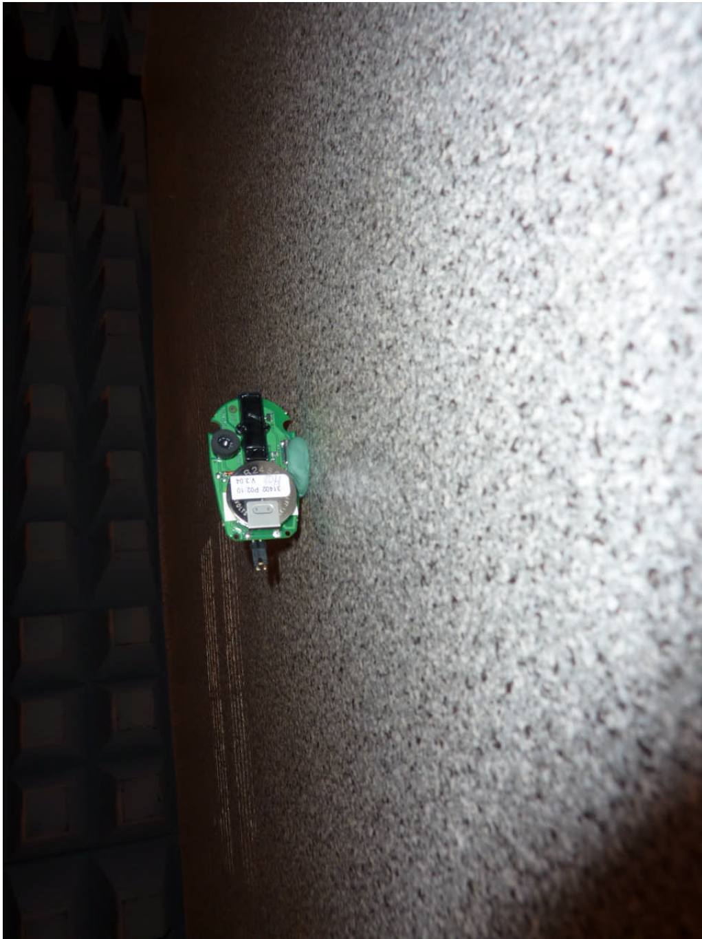
111947_2.JPG: TPU 4030 without housing, test setup fully anechoic chamber (pos. 2)
