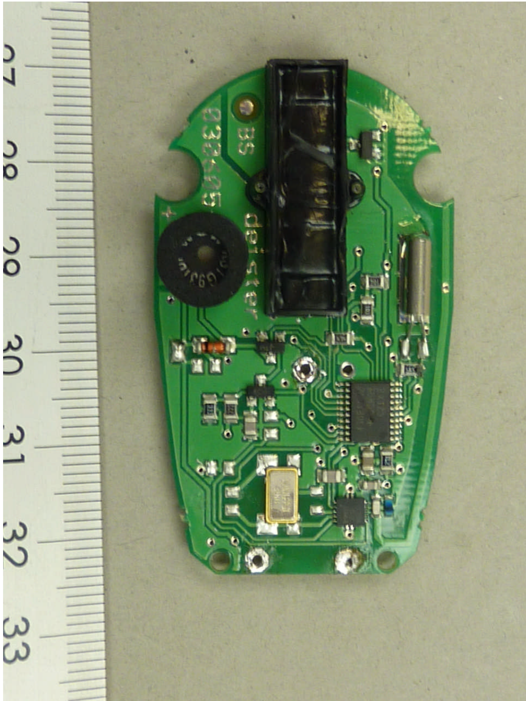
111947_g.JPG: TPU 4030, PCB, top view, battery removed
