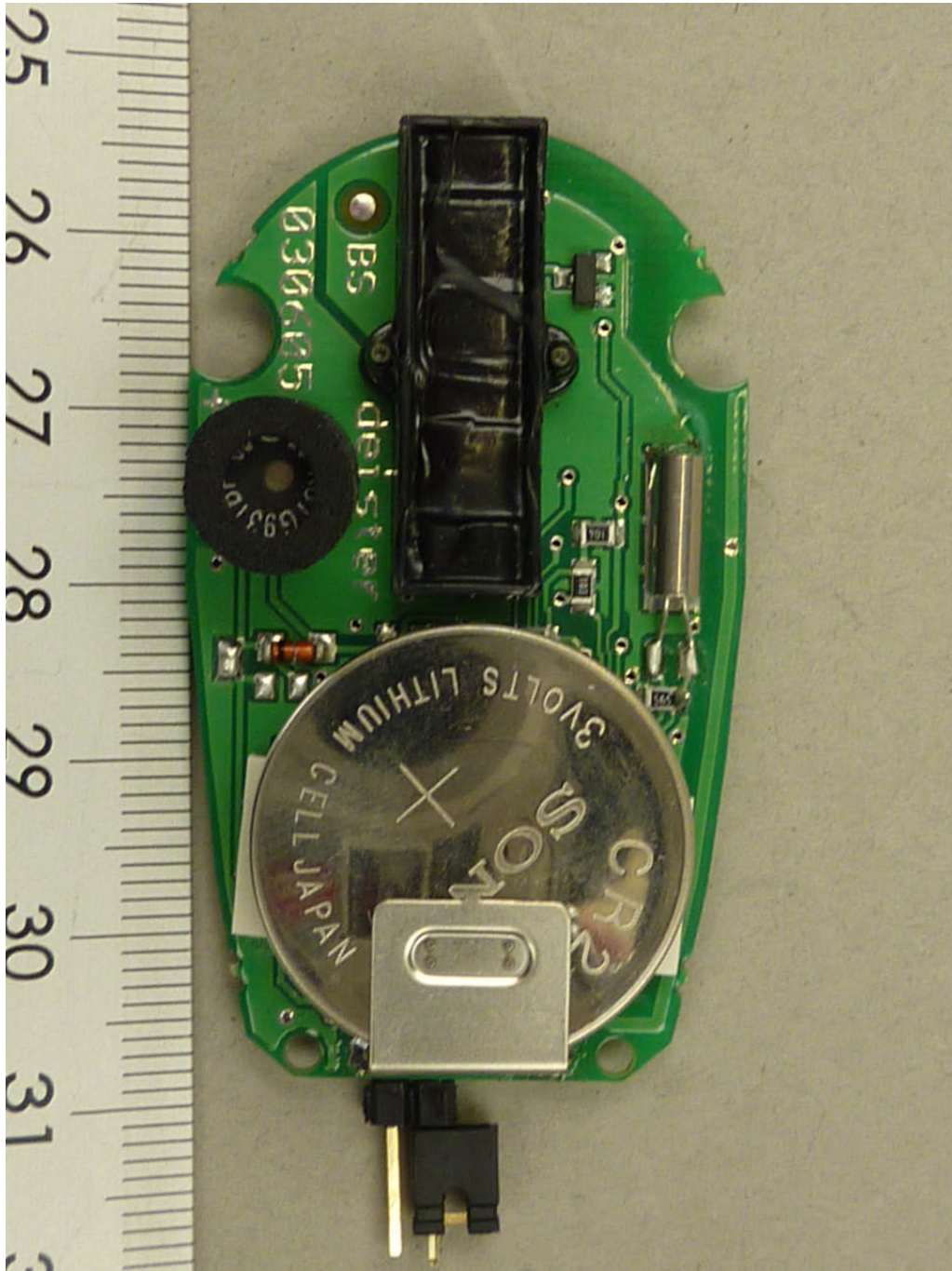
111947_e.JPG: TPU 4030, PCB, top view
