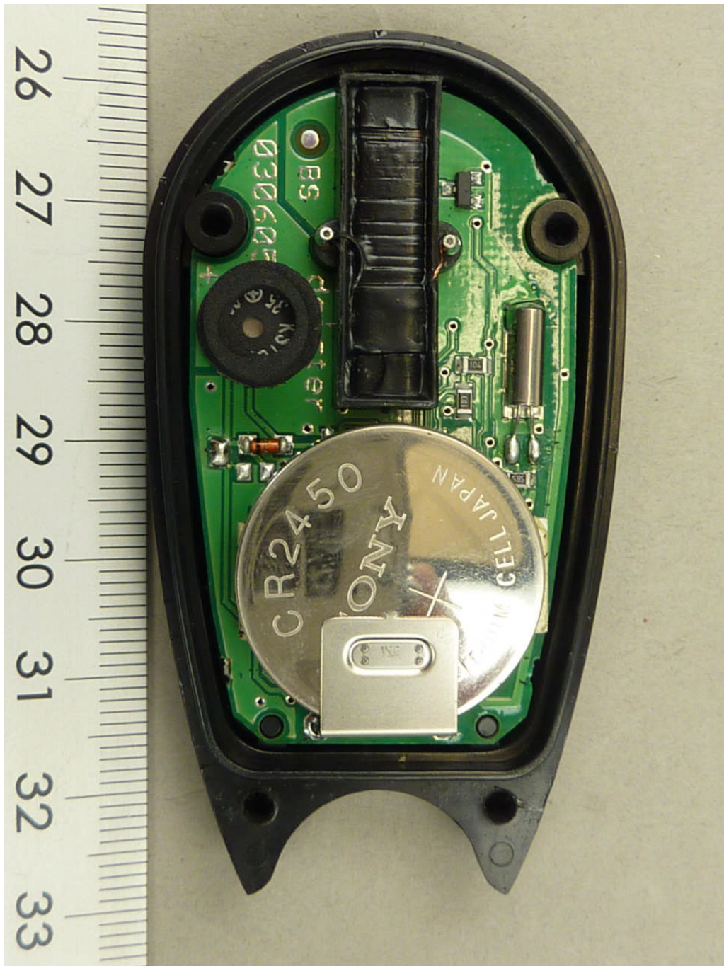
111947_h.JPG: TPU 4030 internal view
