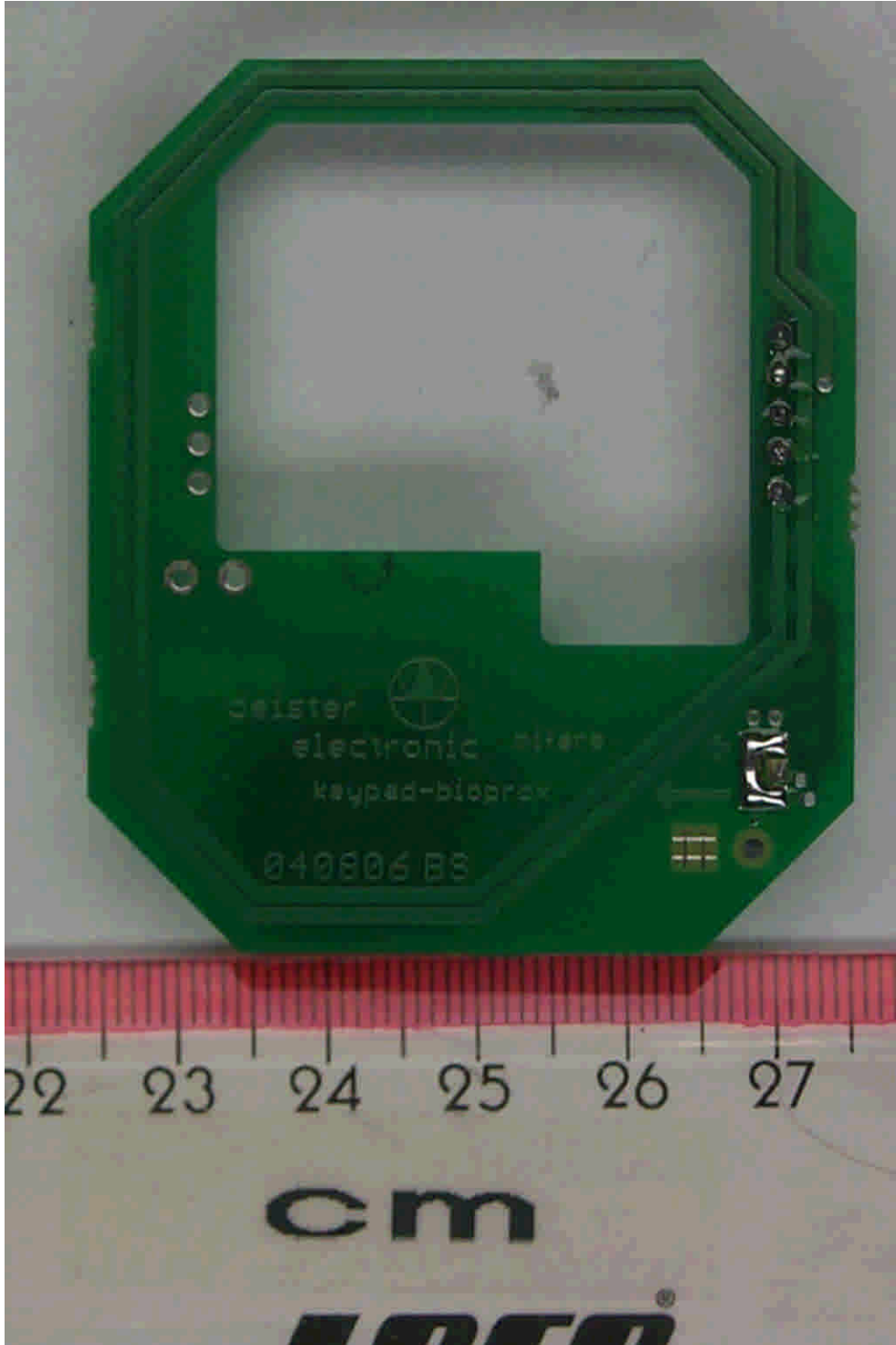
41092A_a.jpg PRM5 / SWH-2100, antenna PCB, bottom view
