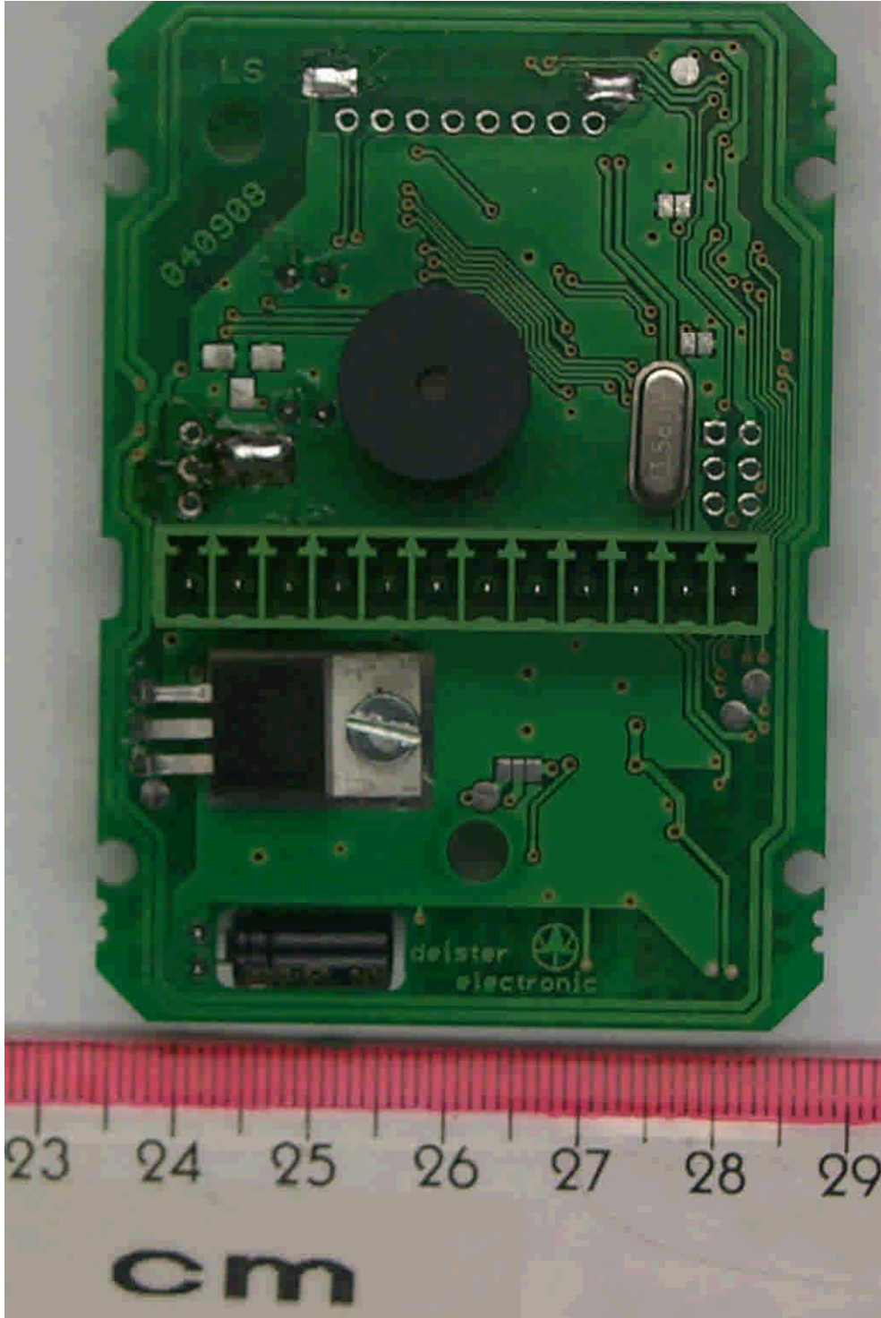
41092A_c.jpg PRM5 / SWH-2100, main PCB, top view
