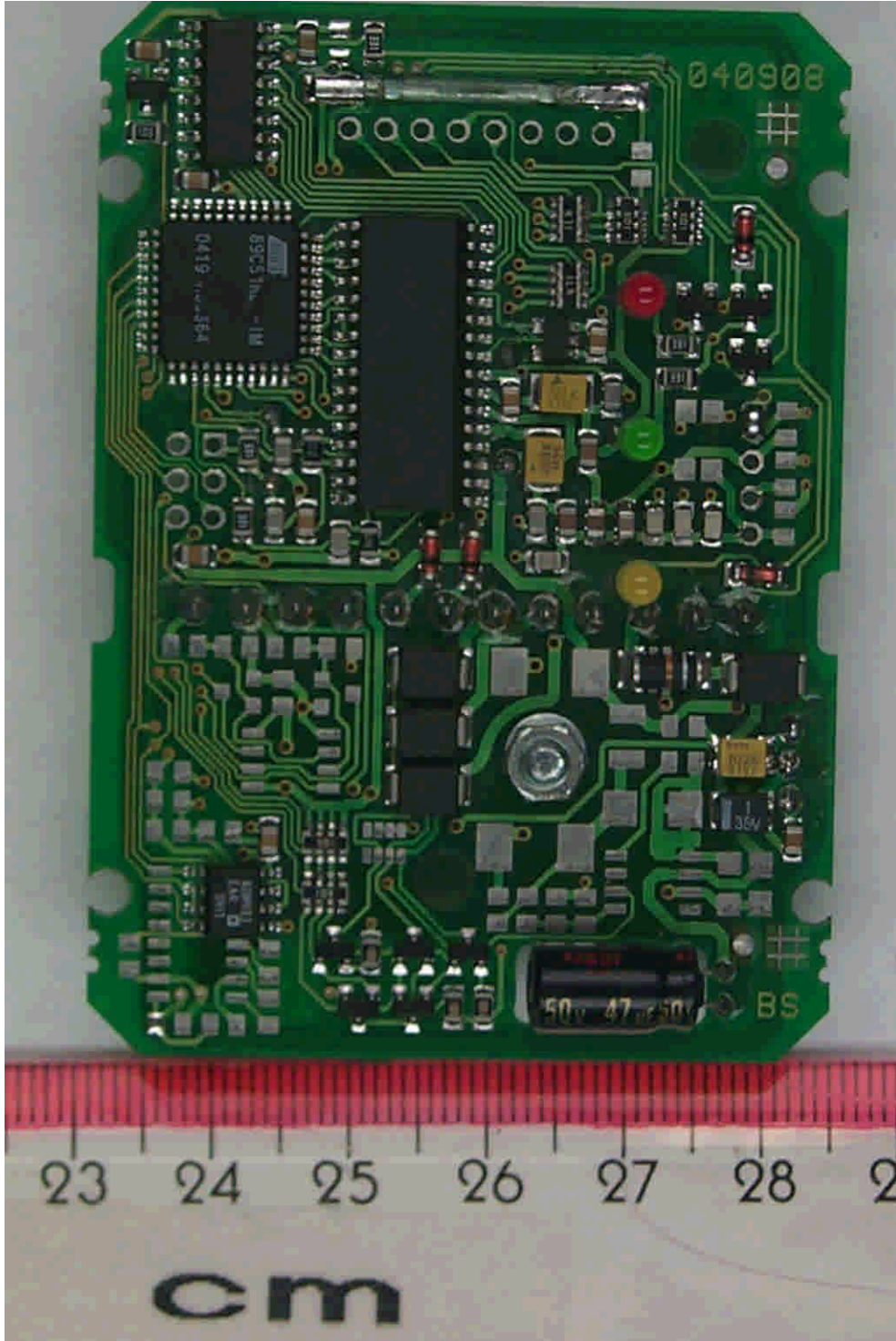
41092A_b.jpg PRM5 / SWH-2100, main PCB, bottom view
