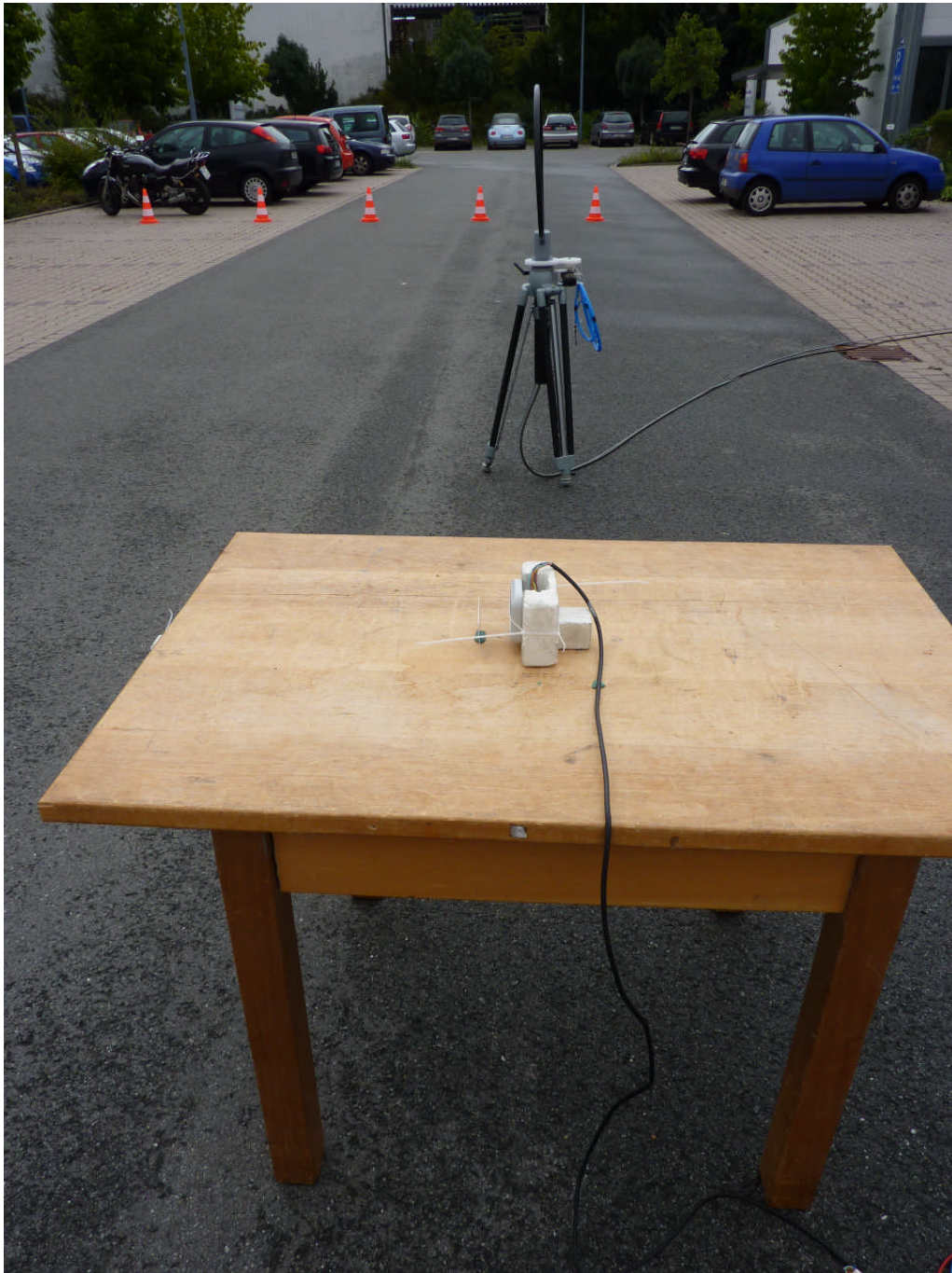
113050_j.JPG: PRL5A/2, test setup outdoor test site
