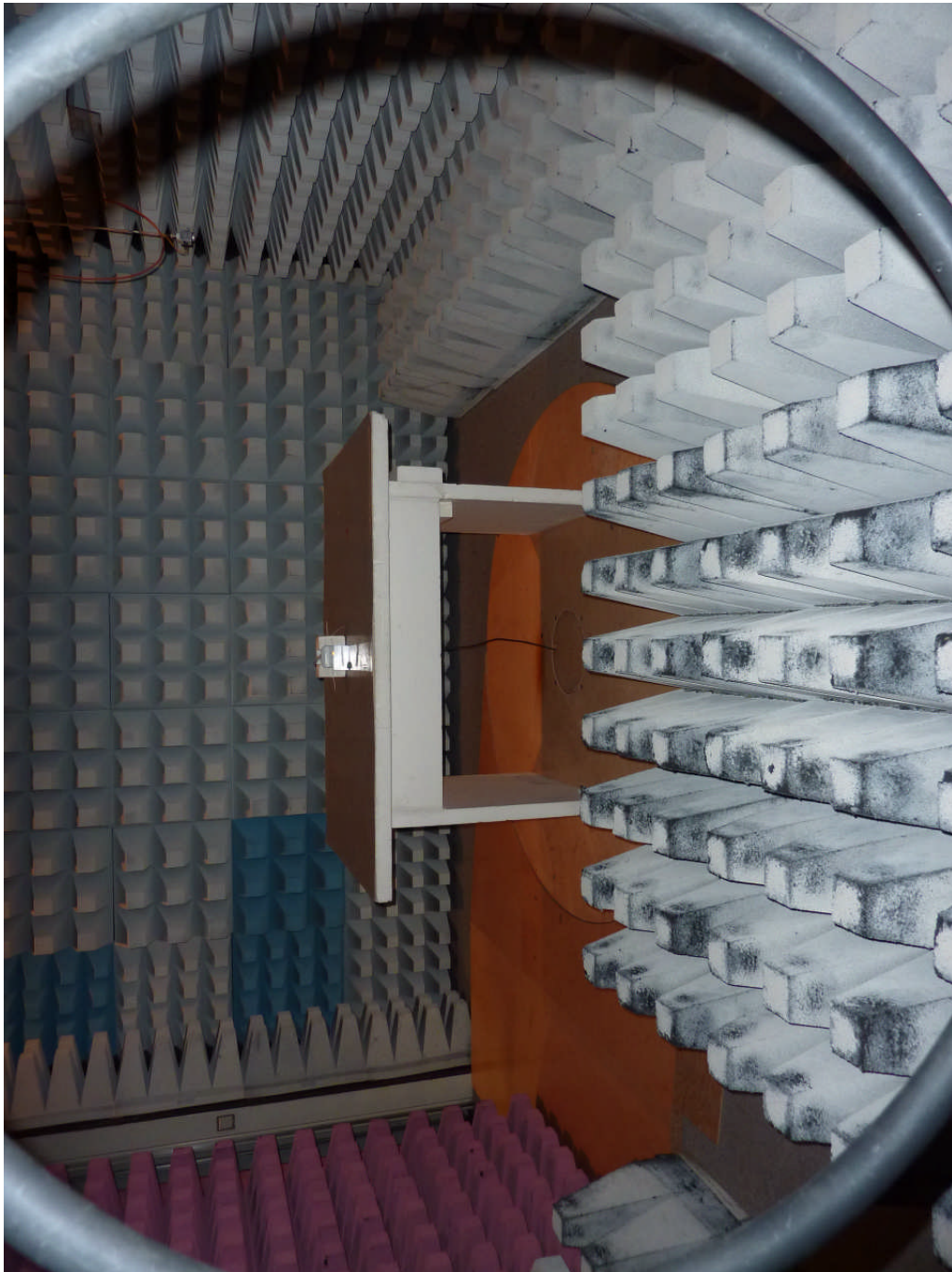
113050_a.JPG: PRL5A/2, test setup fully anechoic chamber
