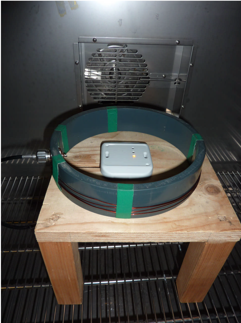
113050_k.JPG: PRL5A/2, test setup climatic chamber
