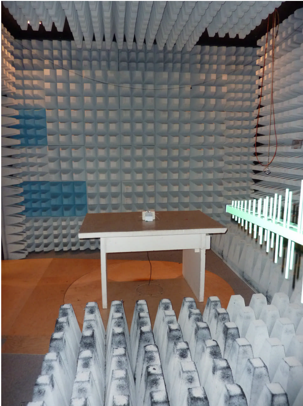
113050_e.JPG: PRL5A/2, test setup fully anechoic chamber
