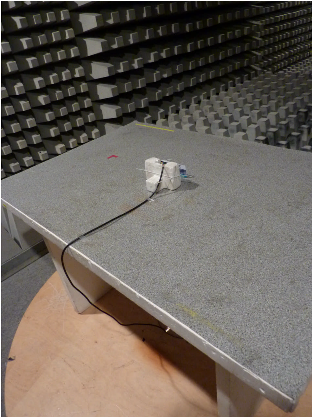
113050_c.JPG: PRL5A/2, test setup fully anechoic chamber
