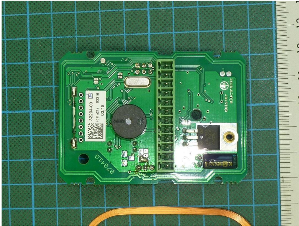
181073eut25: PRD5/2 PCB2 bottom view
