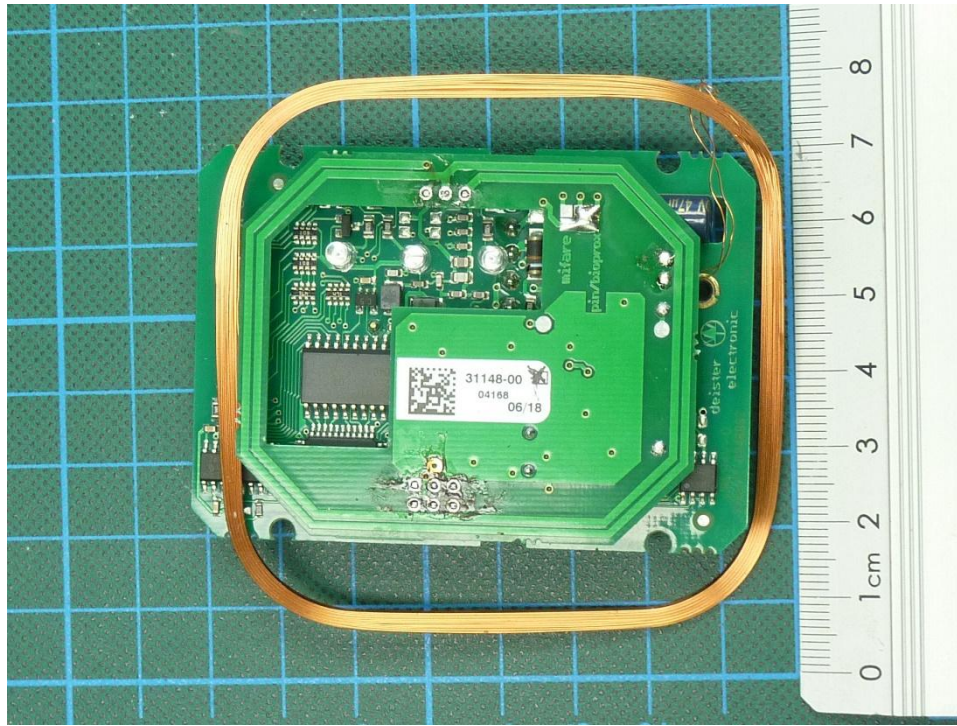
181073eut21: PRD5/2 EUT inside view 3
