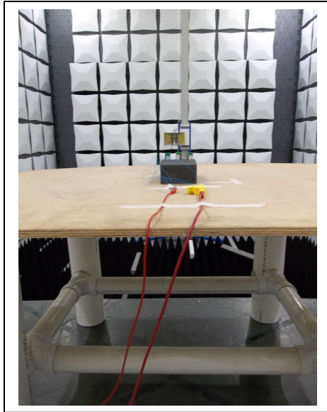
Loop Antenna
