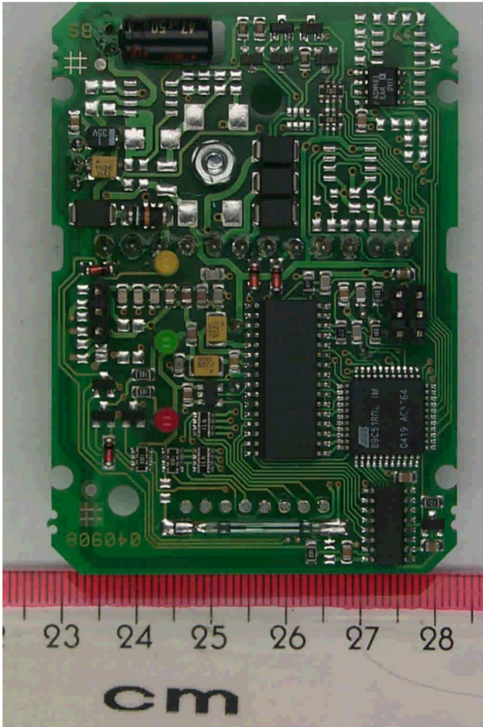
41092C_c.jpg KPD5 / SWH-4200, main PCB, bottom view
