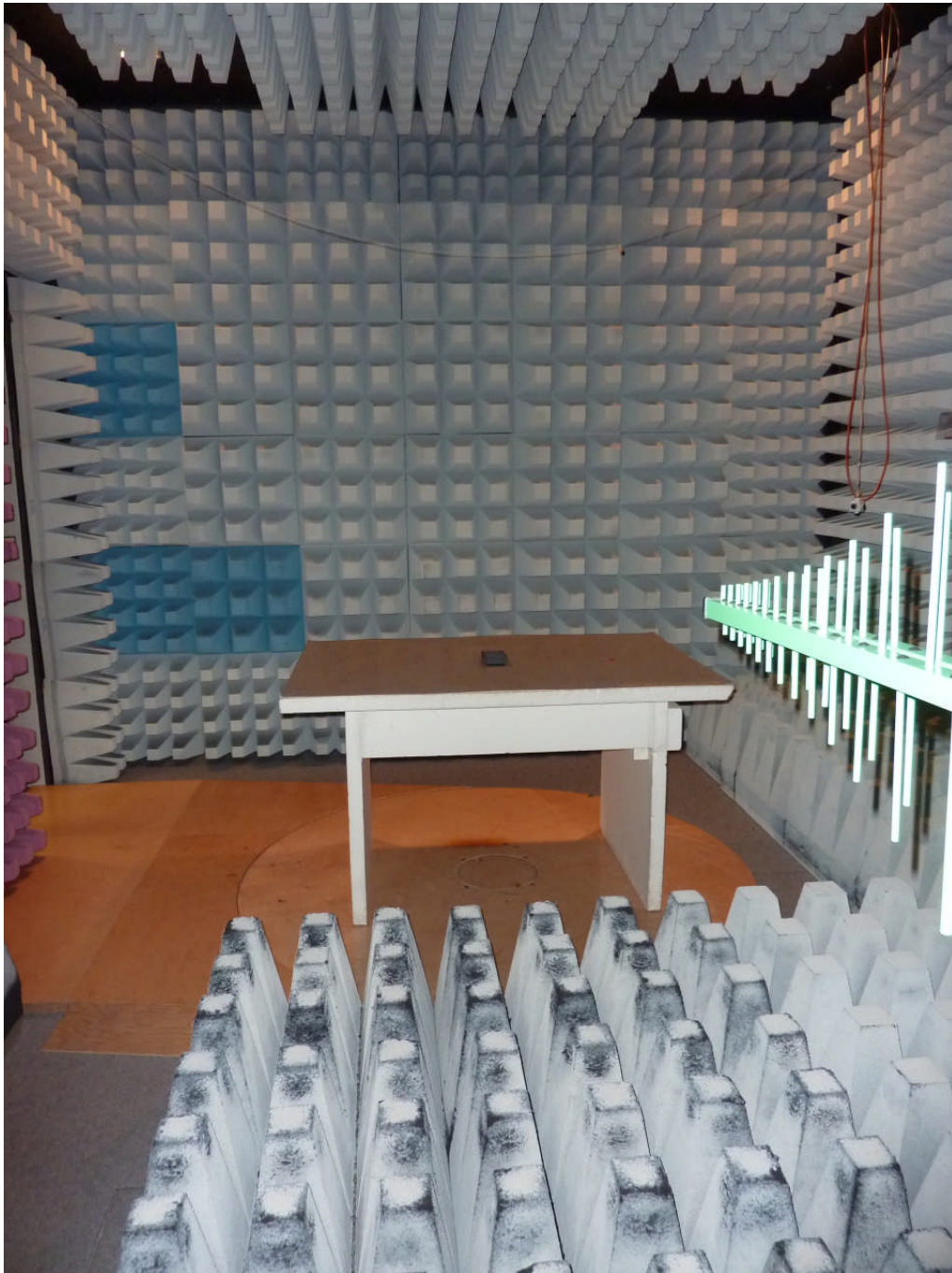
111946_5.JPG: ADA Amantag Deactivator without TAG, test setup fully anechoic chamber (pos. 1)
