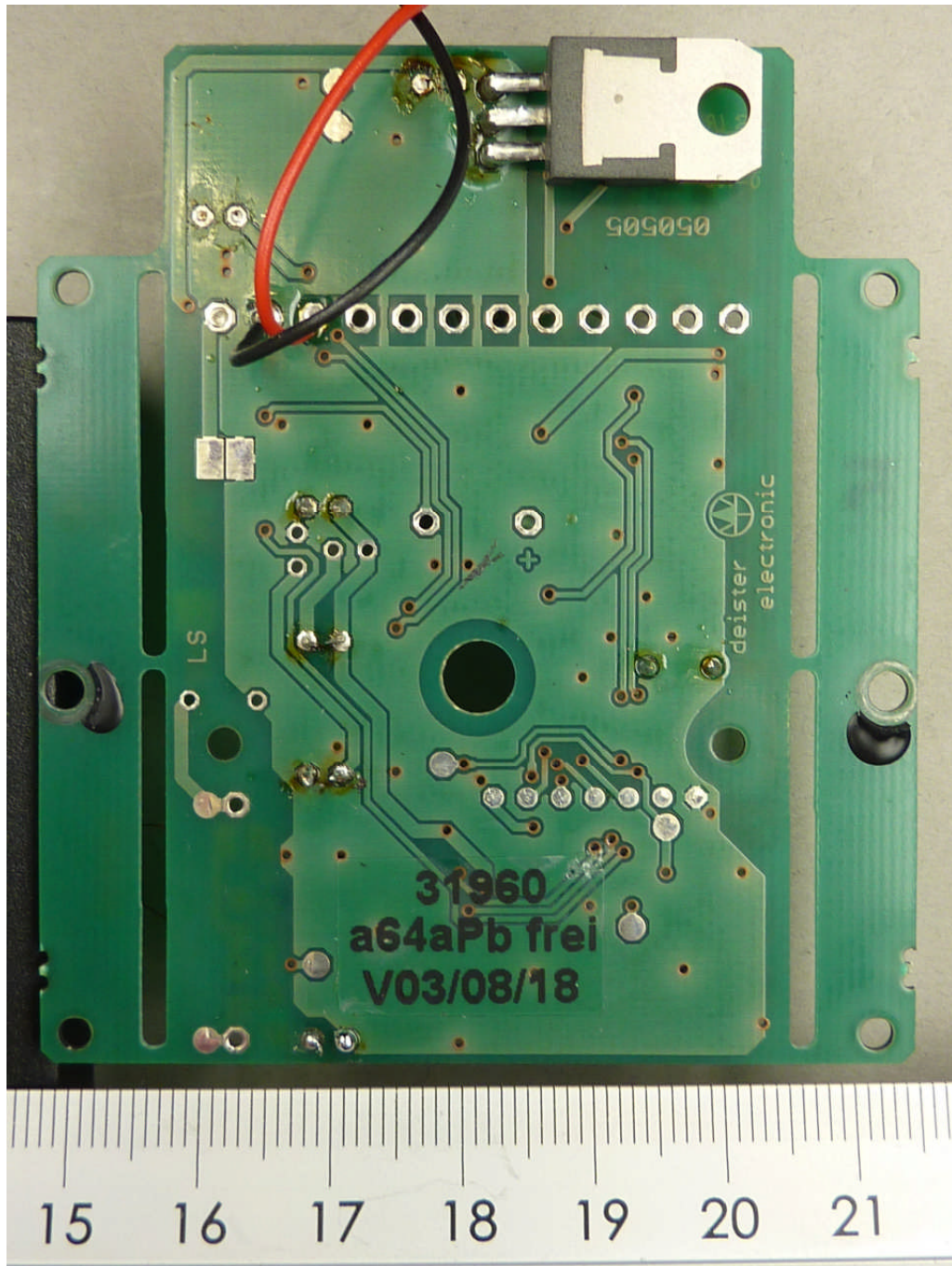
111946_g.JPG: ADA Amantag Deactivator, PCB, bottom view
