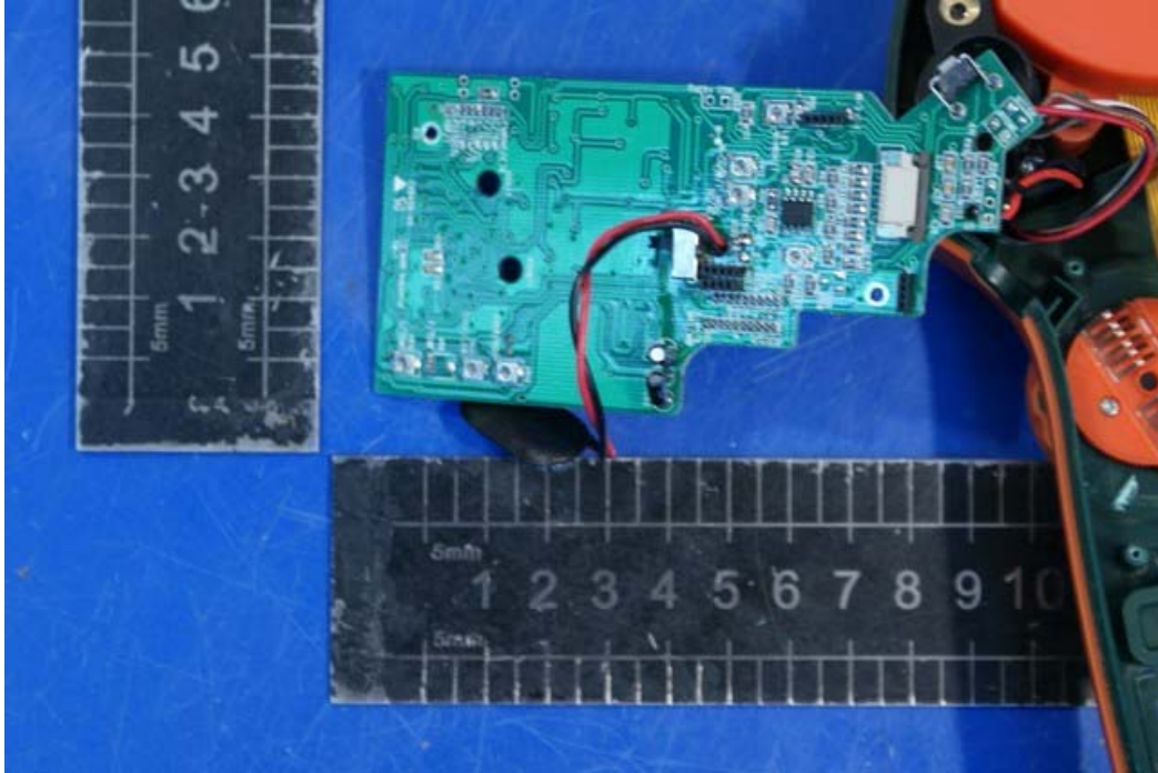
Photo 7 Inside of EUT
