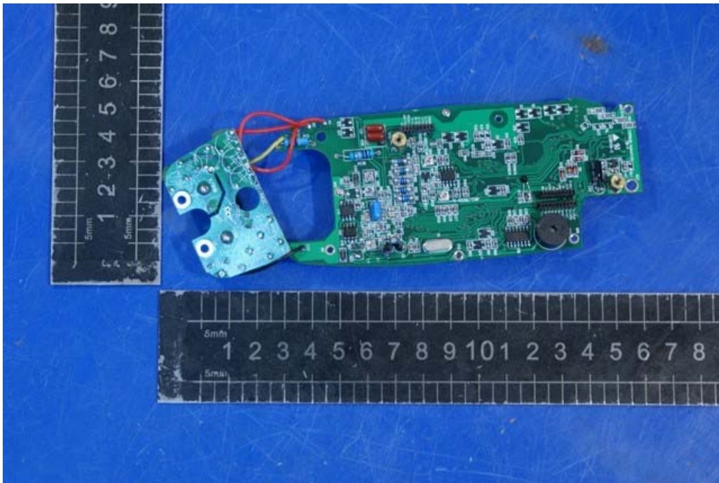
Photo 4 Inside of EUT
