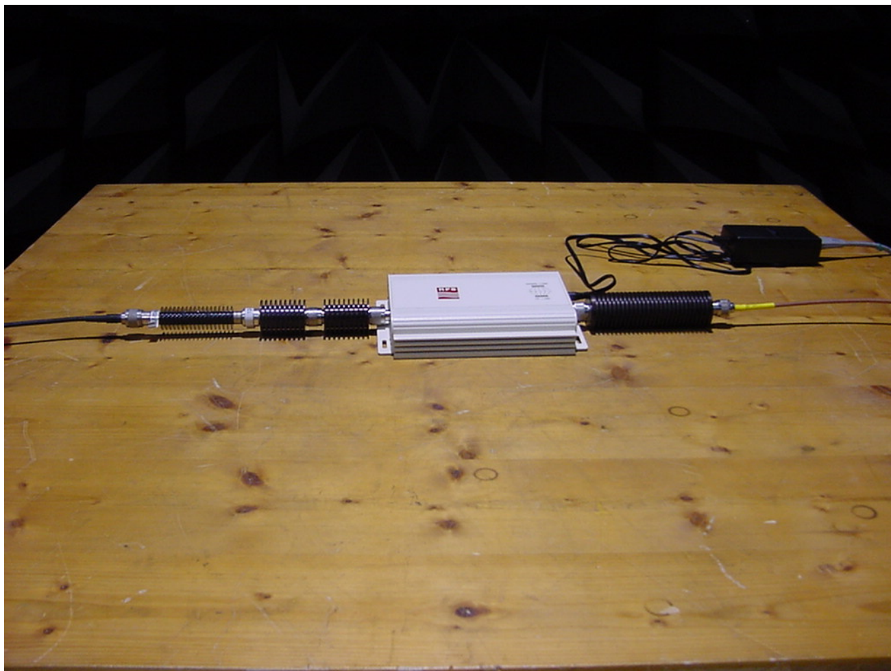
Photo 2: Radiated Emissions
