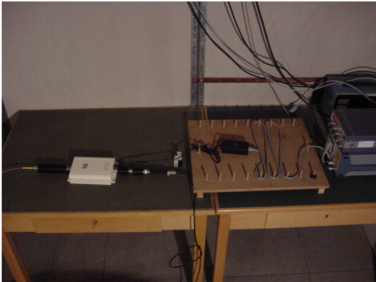
Photo 3: Conducted Emissions
