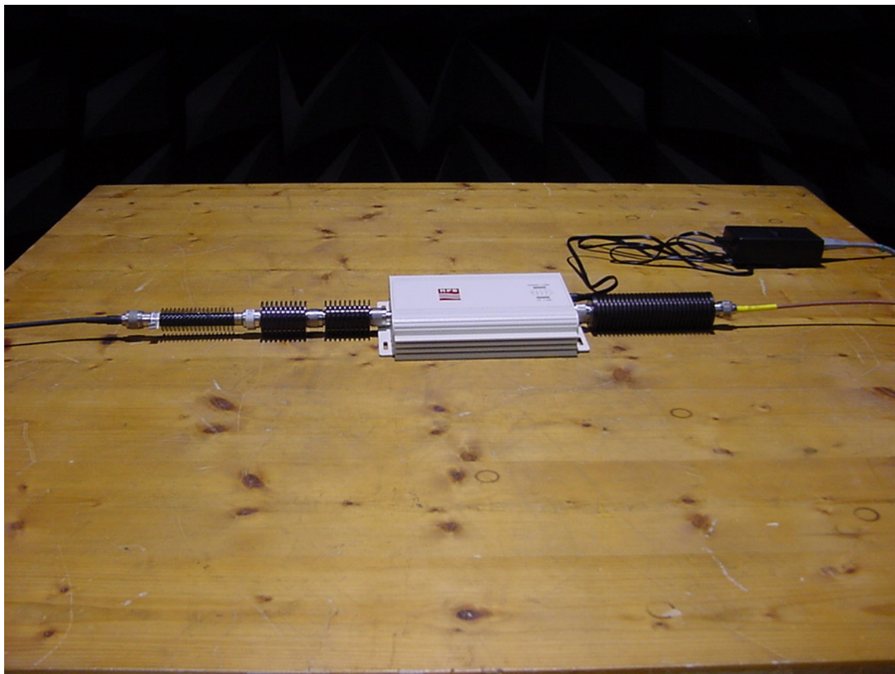
Photo 2: Radiated Emissions
