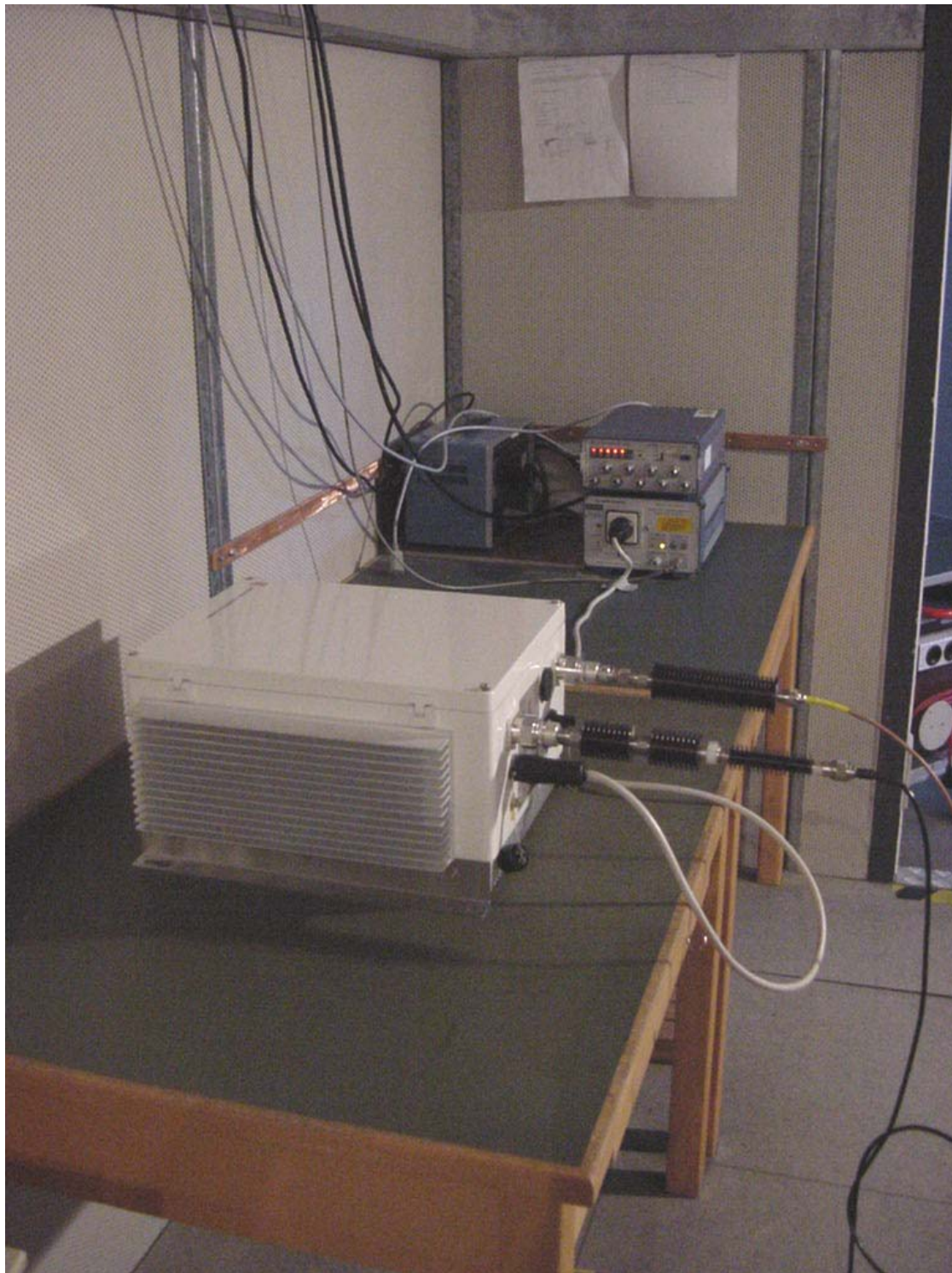
Photo 3: Conducted Emissions
