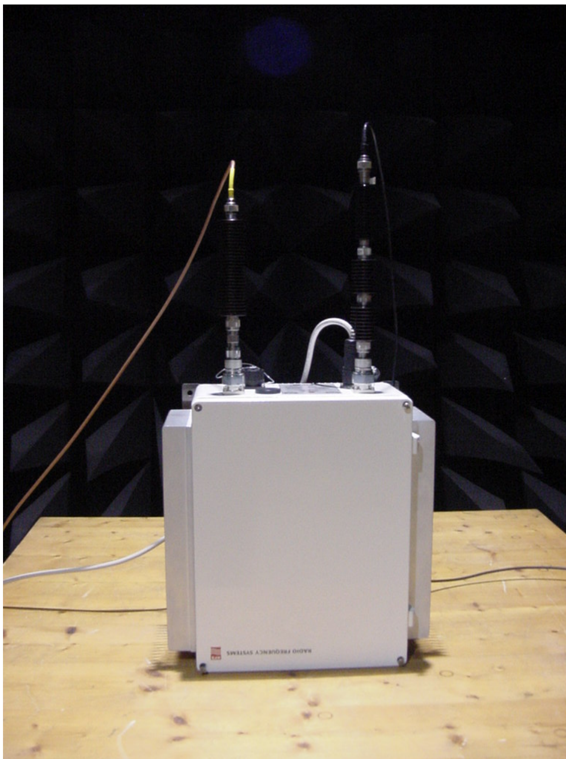
Photo 2: Radiated Emissions
