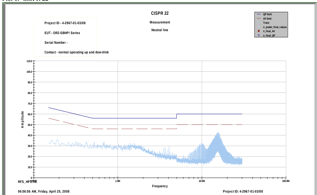
Plot 1: CISPR 22
