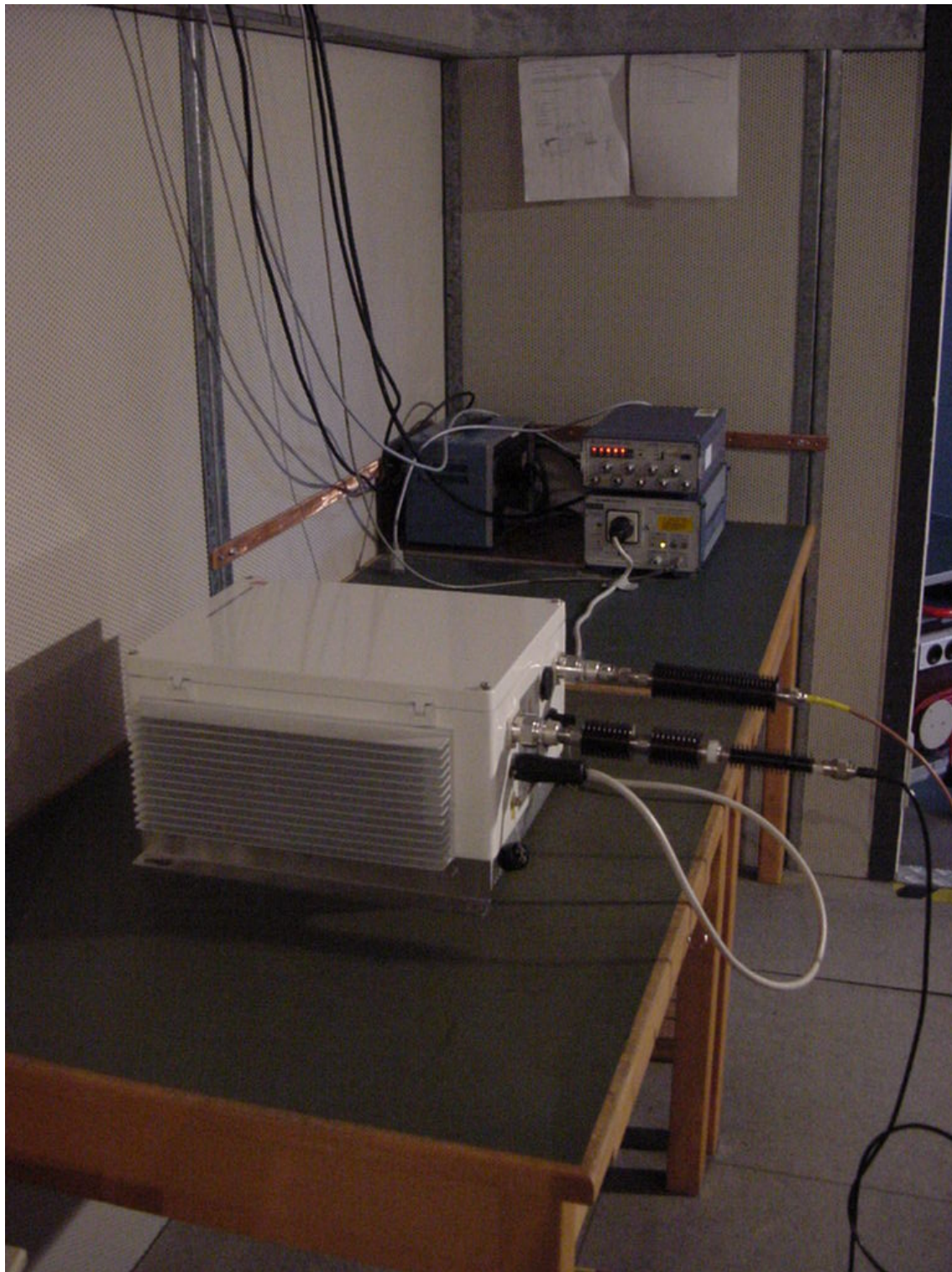
Photo 3: Conducted Emissions
