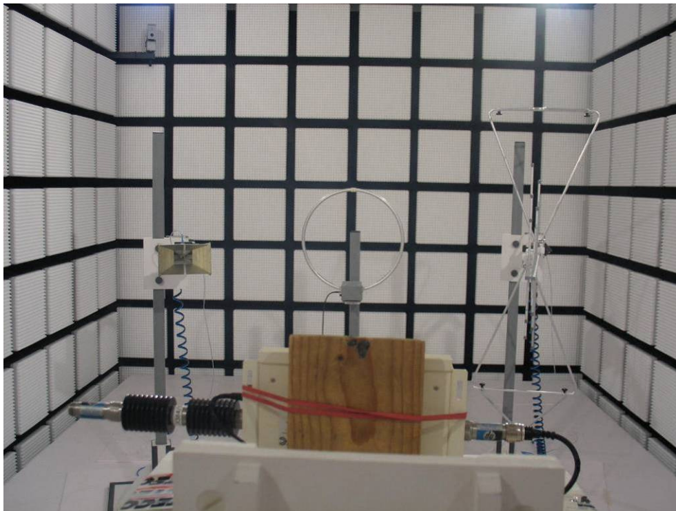
Photo 3: Radiated Emissions
