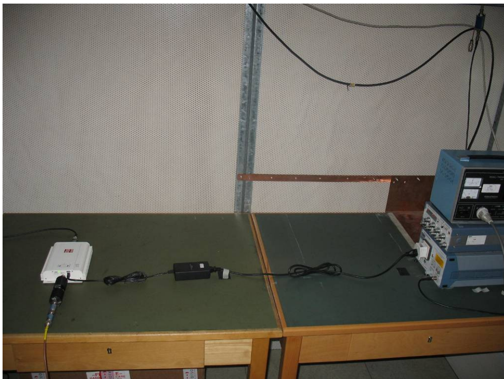
Photo 4: Conducted Emissions
