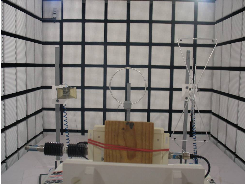
Photo 3: Radiated Emissions
