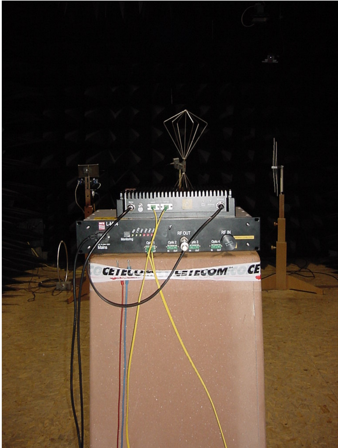
Photo 2: Radiated Emissions
