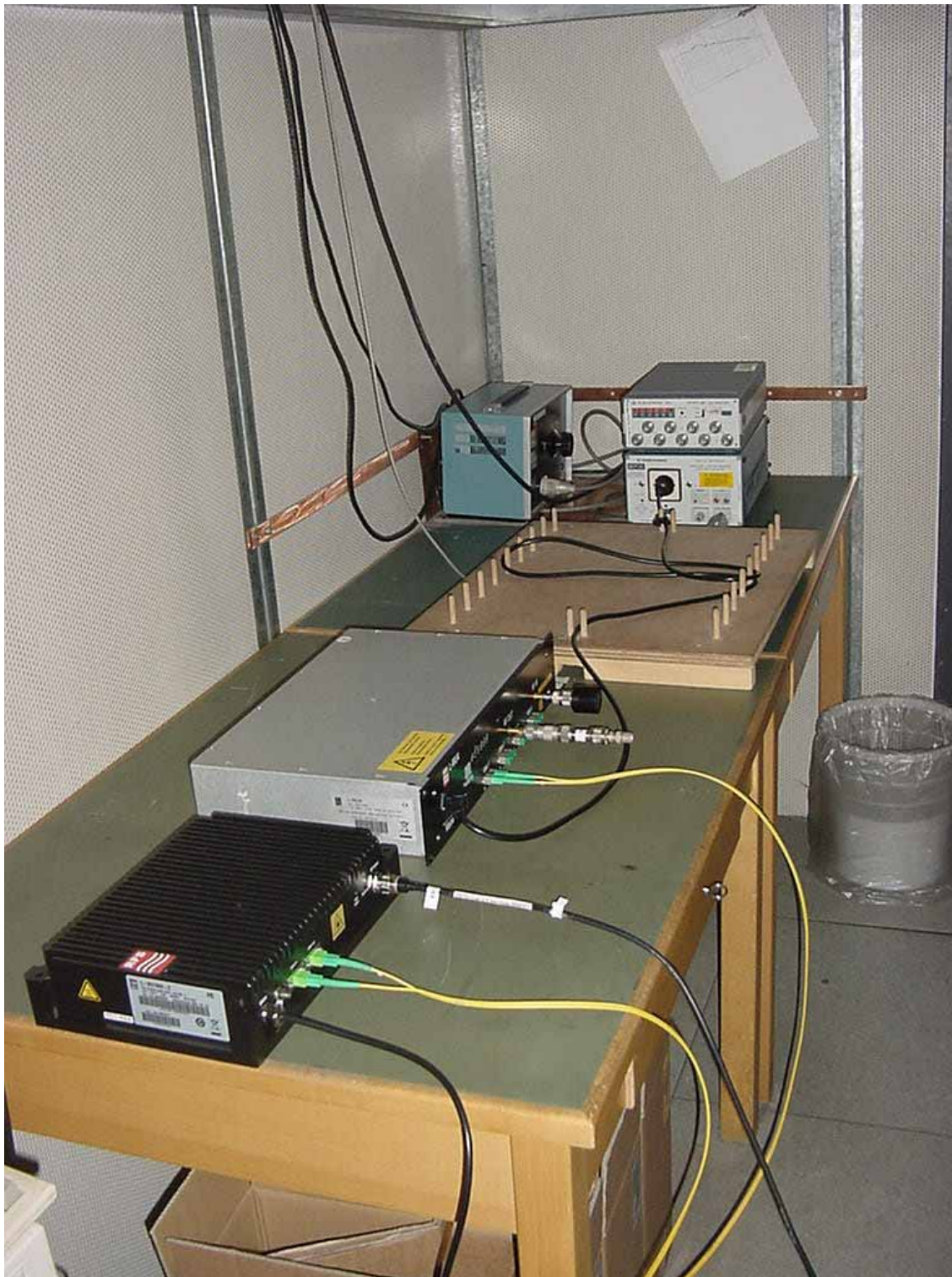
Photo 3: Conducted Emissions
