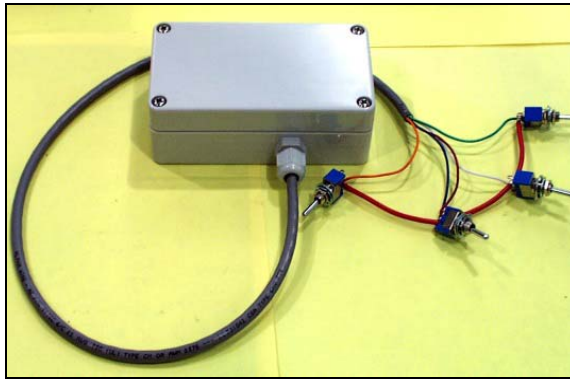
PowerTouch 1800-TIM-TW4 Transmitter in case – Top View
