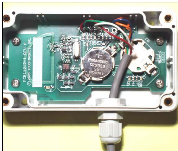
PowerTouch 1800-TIM-TW4 Transmitter PCB – Top View
