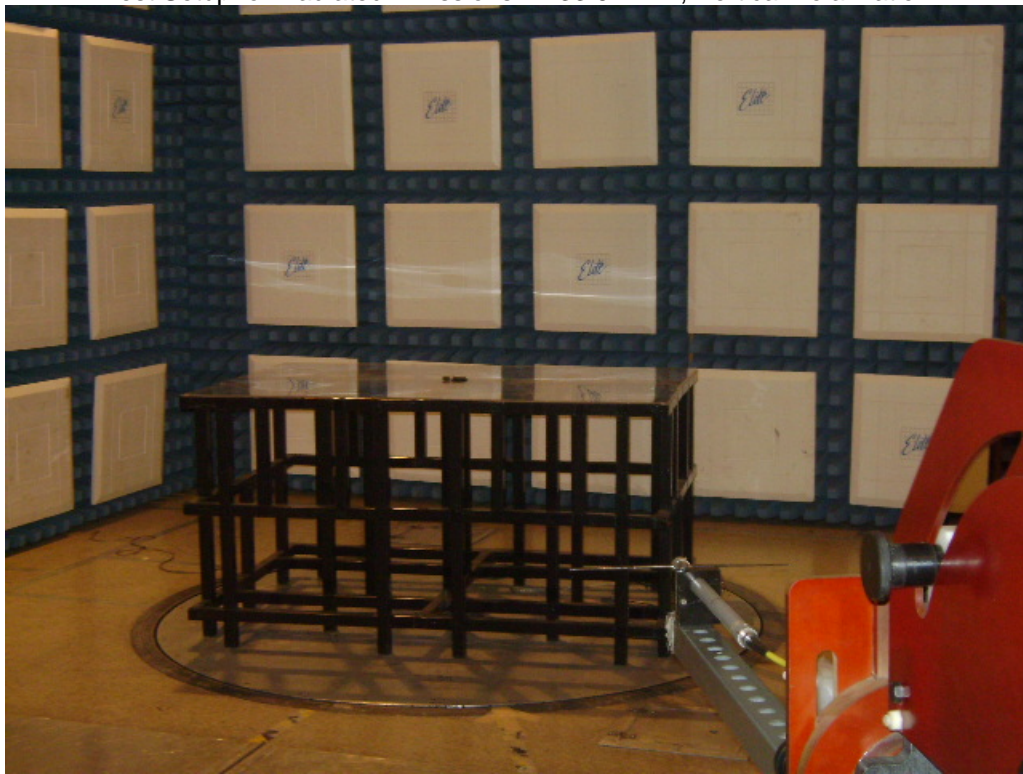
Test Setup for Radiated Emissions – 433.92MHz, Horizontal Polarization
