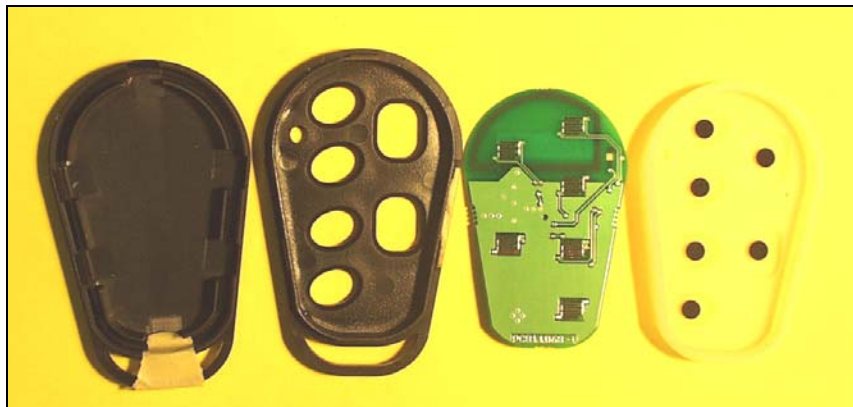
PowerTouch PowerTouch 1000-TF Transmitter in case – Top View
