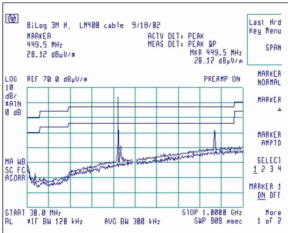
Graph of scan made in shielded enclosure
