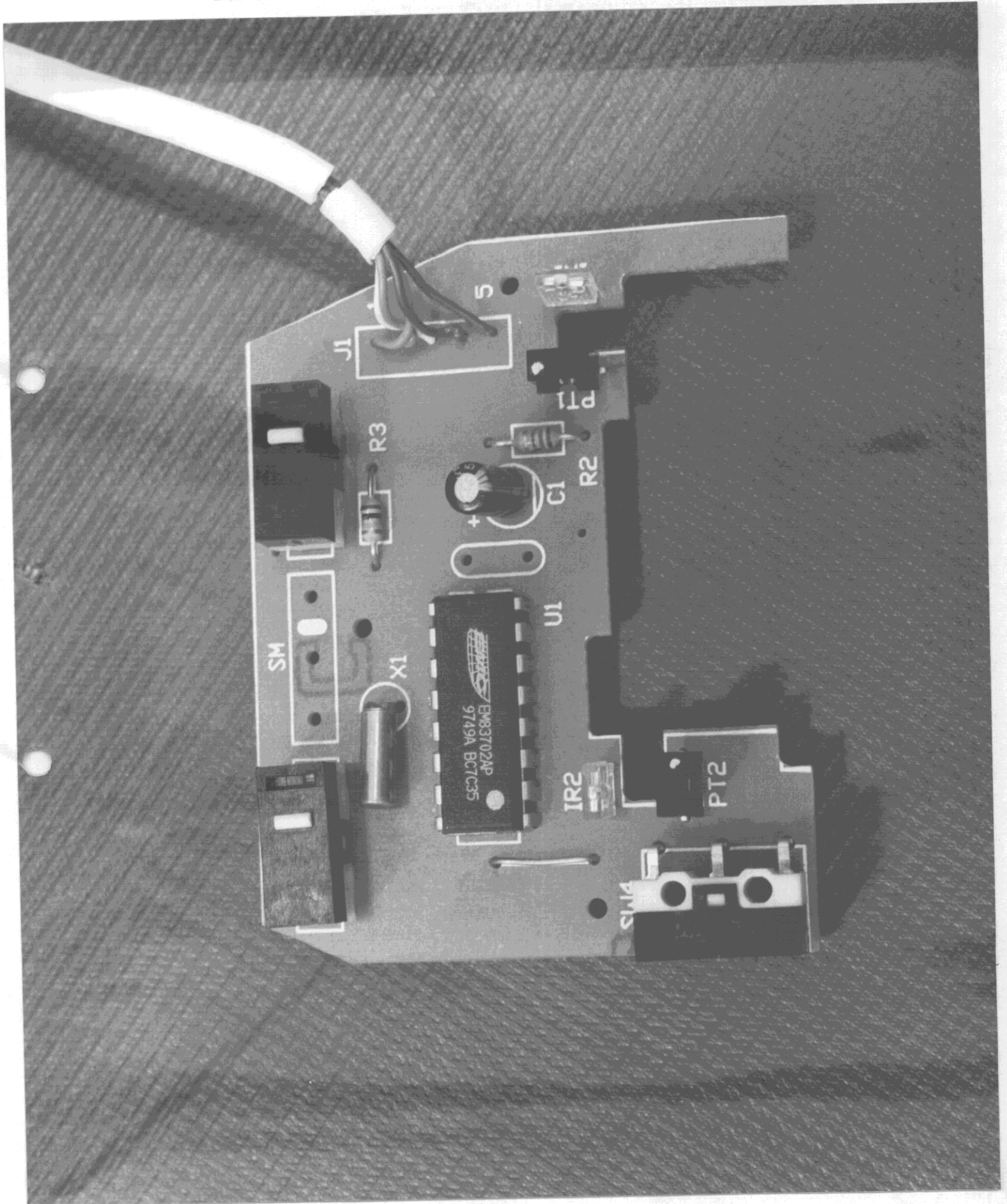
PHOTO 4. EUT COMPONENT SIDE VIEW
