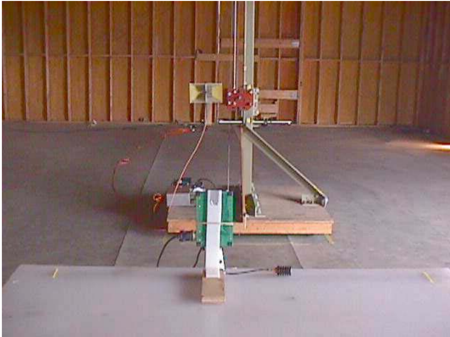
PHOTO #5 OF 6 VERTICAL TO RECEIVING ANTENNA – FRONT VIEW
