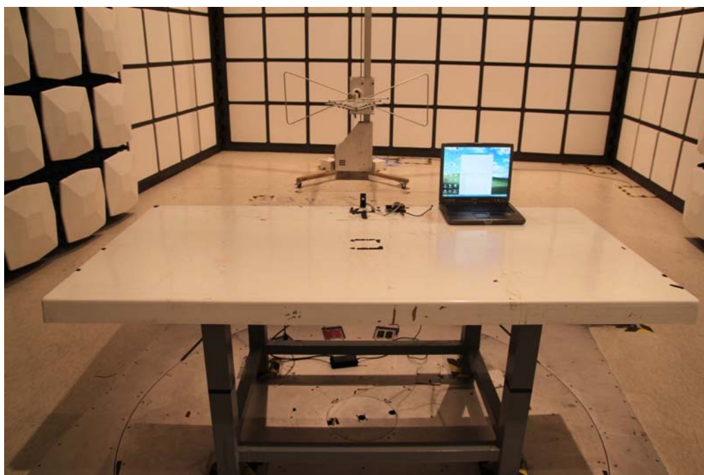
Front View
