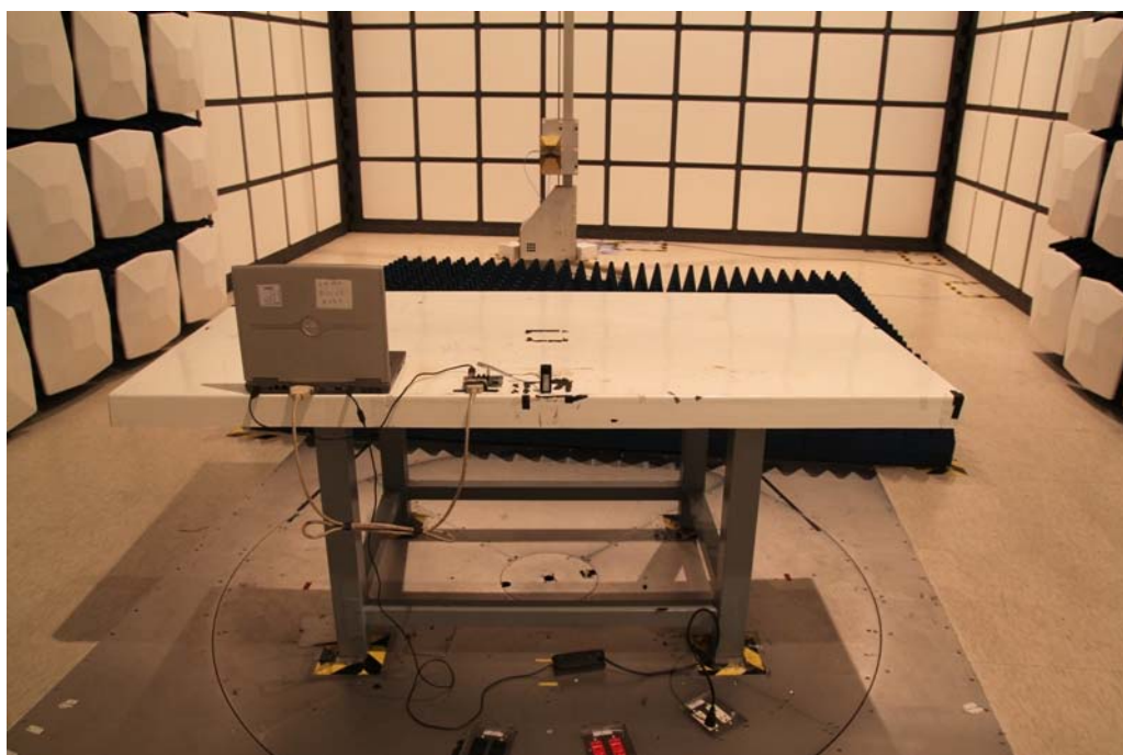
Rear View
