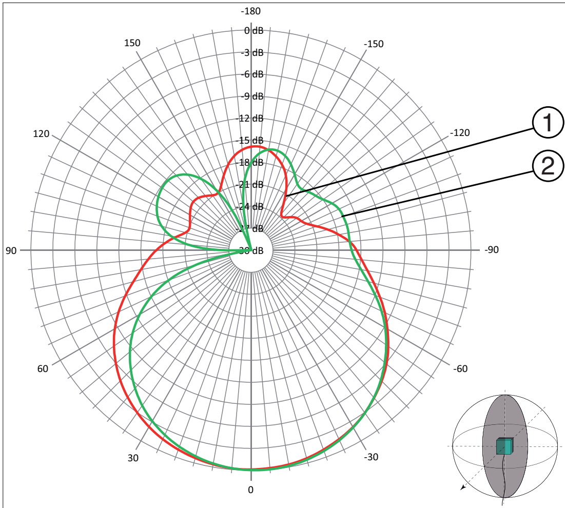
Figure 10.3 ① - Horizontal polarization ② - Vertical polarization
