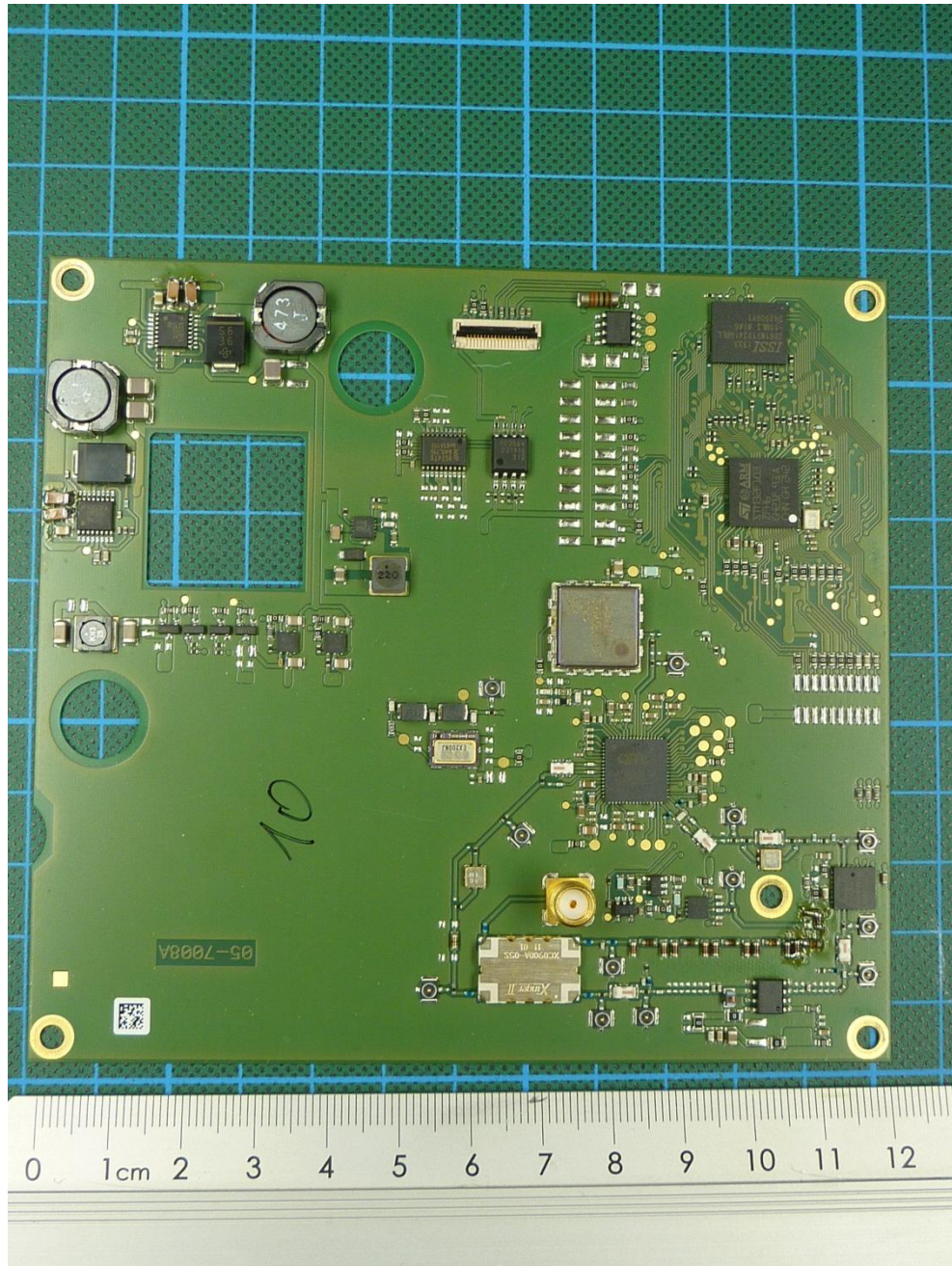
152117_7.JPG: IUH-F192-V1-FR2-02, PCB 1, top view
