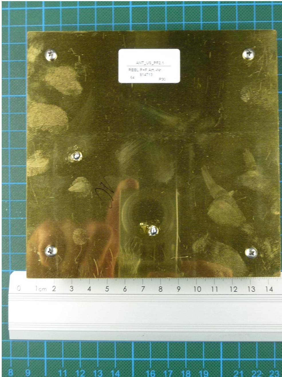
152117_13.JPG: IUH-F192-V1-FR2-02, antenna, top view
