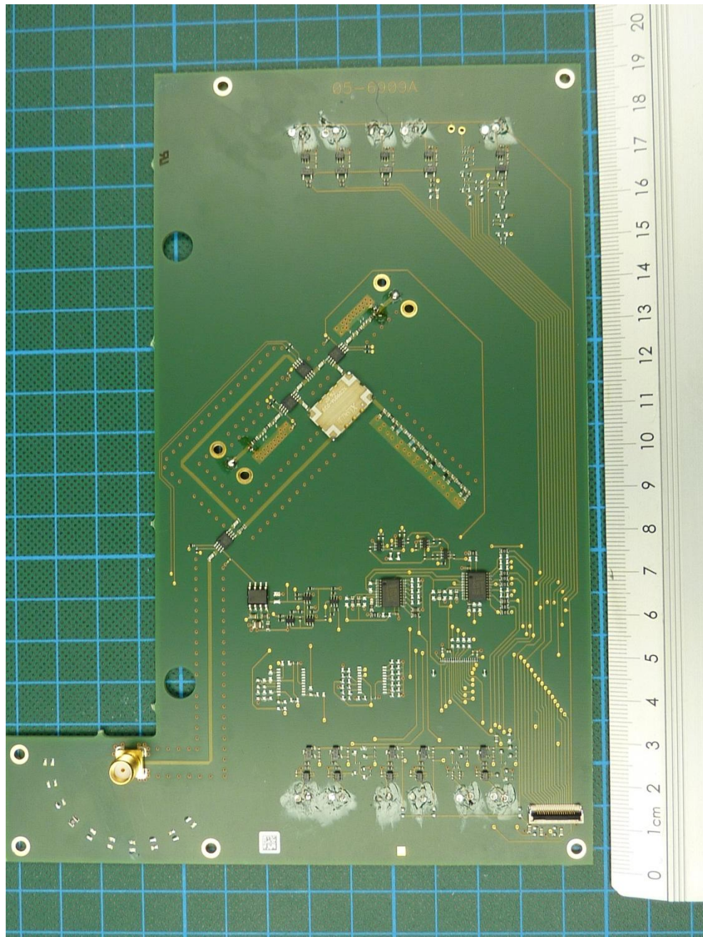
152117_10.JPG: IUH-F192-V1-FR2-02, PCB 3, top view
