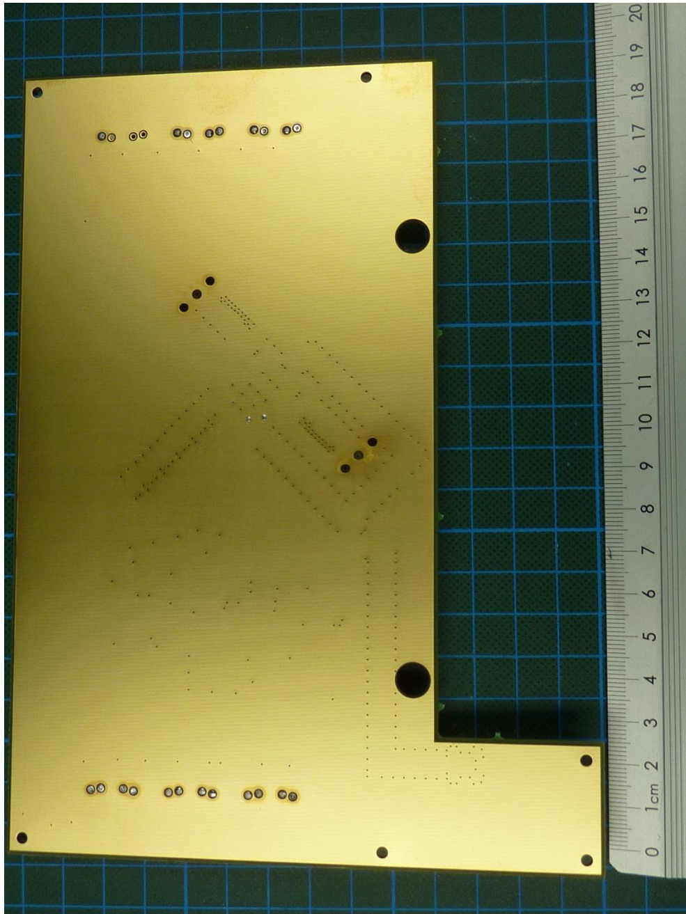
152117_11.JPG: IUH-F192-V1-FR2-02, PCB 3, bottom view
