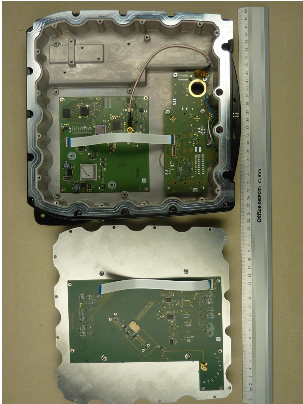
152117_5.JPG: IUH-F192-V1-FR2-02, internal view
