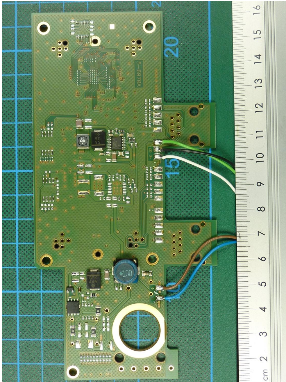
152117_9.JPG: IUH-F192-V1-FR2-02, PCB 2, bottom view
