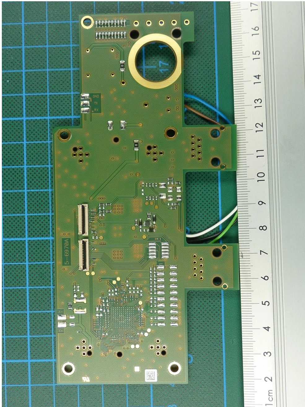
152117_8.JPG: IUH-F192-V1-FR2-02, PCB 2, top view
