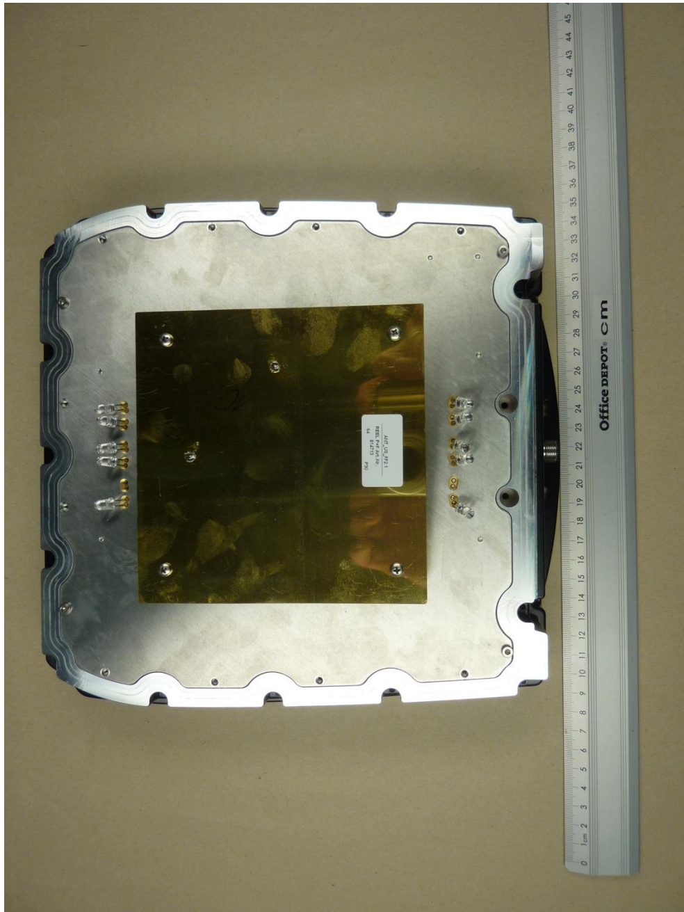
152117_4.JPG: IUH-F192-V1-FR2-02, cover removed
