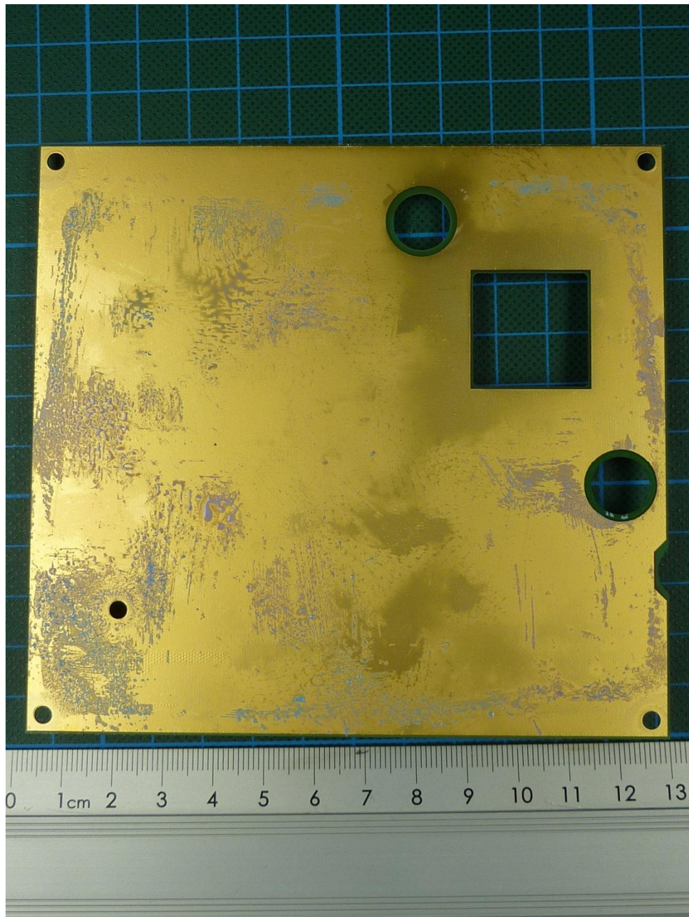
152117_6.JPG: IUH-F192-V1-FR2-02, PCB 1, bottom view
