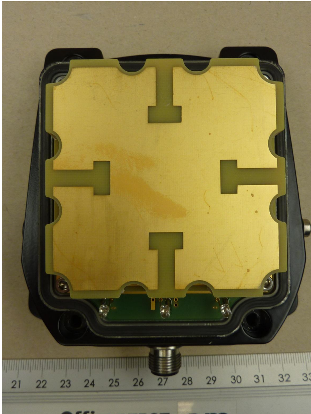
136258_6.JPG: IUH-F190-V1-FR2-02, internal view 2 (front cover removed)
