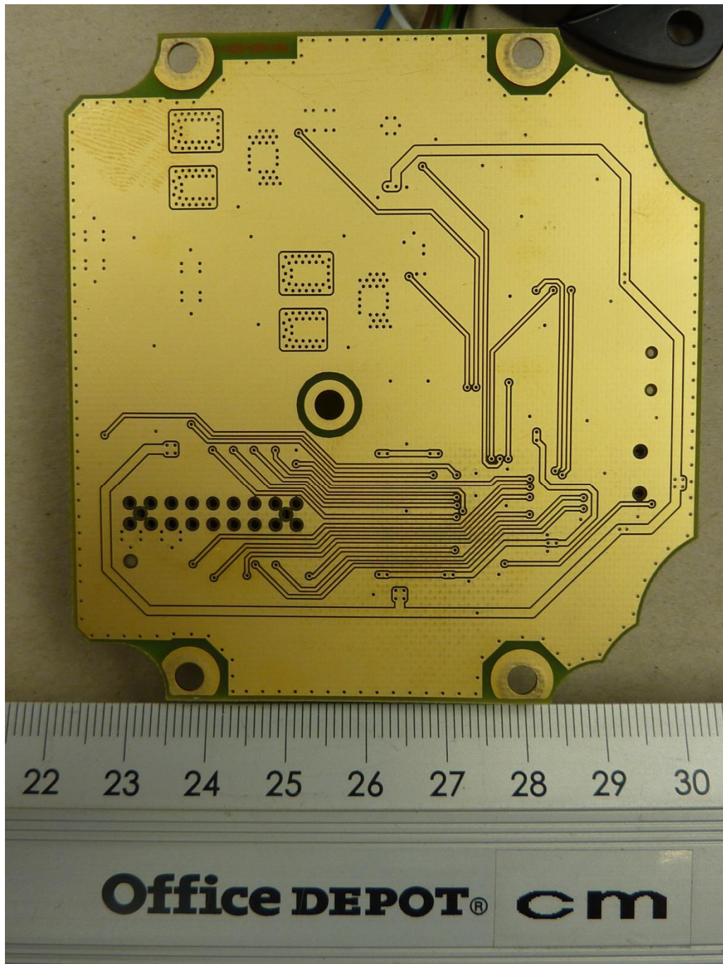
136258_10.JPG: IUH-F190-V1-FR2-02, main PCB, bottom view
