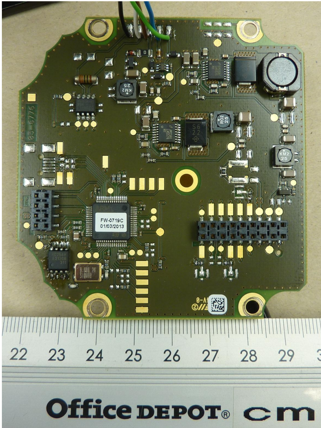
136258_9.JPG: IUH-F190-V1-FR2-02, main PCB, top view
