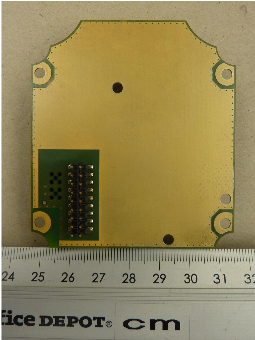
136258_8.JPG: IUH-F190-V1-FR2-02, rf-PCB, bottom view
