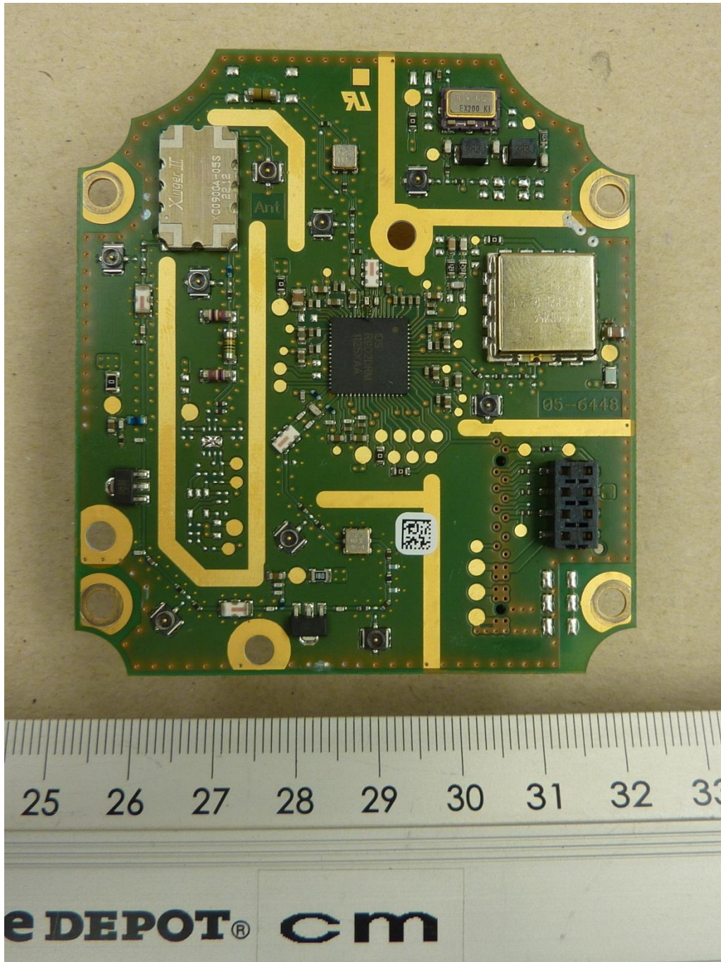
136258_7.JPG: IUH-F190-V1-FR2-02, rf-PCB, top view
