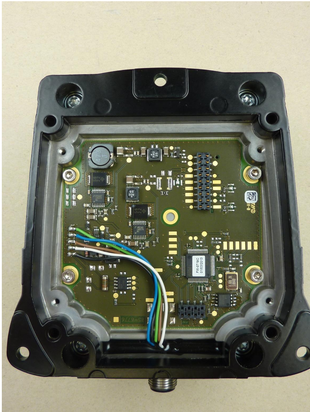
136258_5.JPG: IUH-F190-V1-FR2-02, internal view 1 (rear cover removed)
