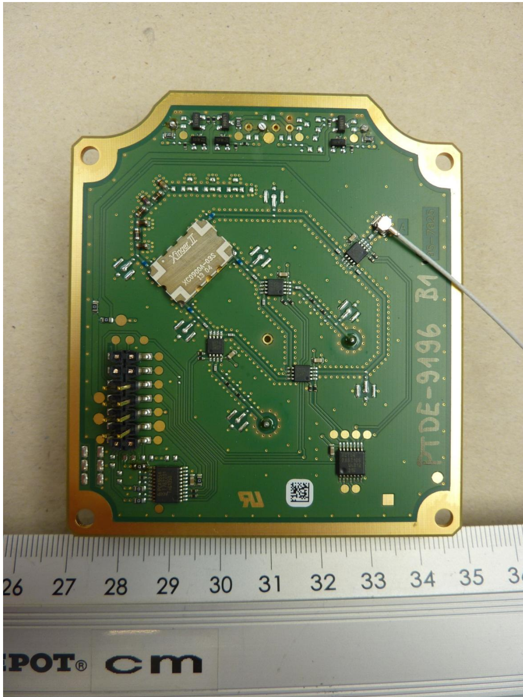
136258_11.JPG: IUH-F190-V1-FR2-02, antenna PCB, bottom view
