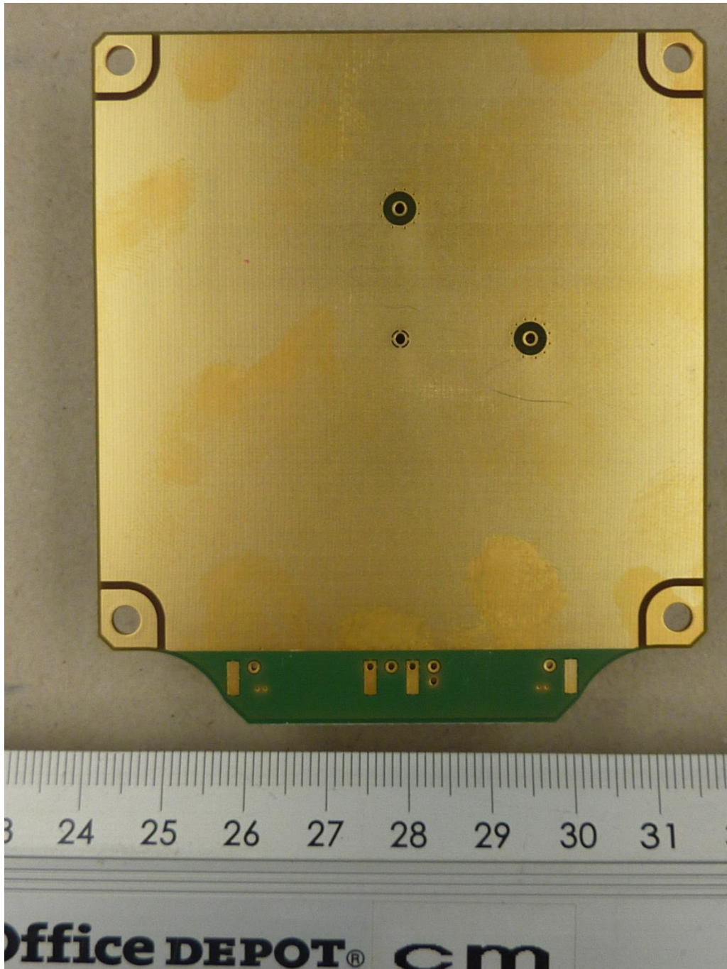
136258_15.JPG: IUH-F190-V1-FR2-02, antenna PCB, top view (antenna removed)
