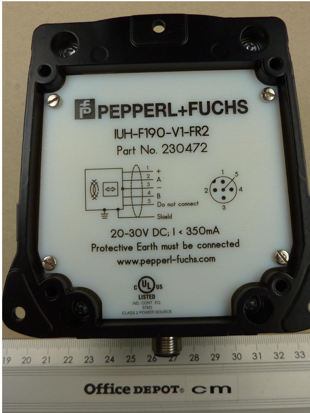
136258_4.JPG: IUH-F190-V1-FR2-02, type plate
