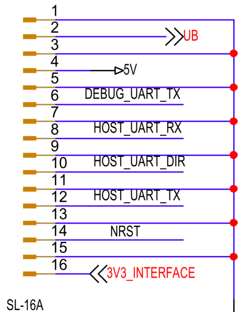
Figure 3 Pinning of module to host connection
