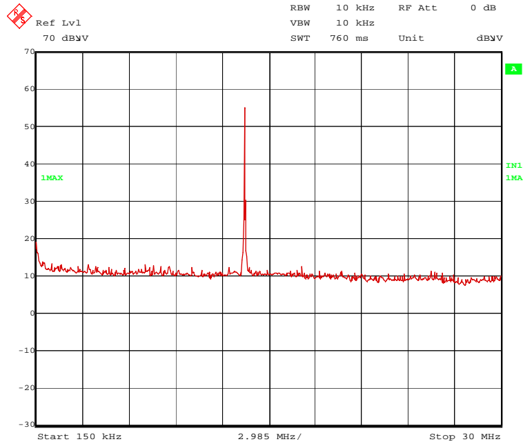
134118b.wmf: Spurious emissions from 150 kHz to 30 MHz
