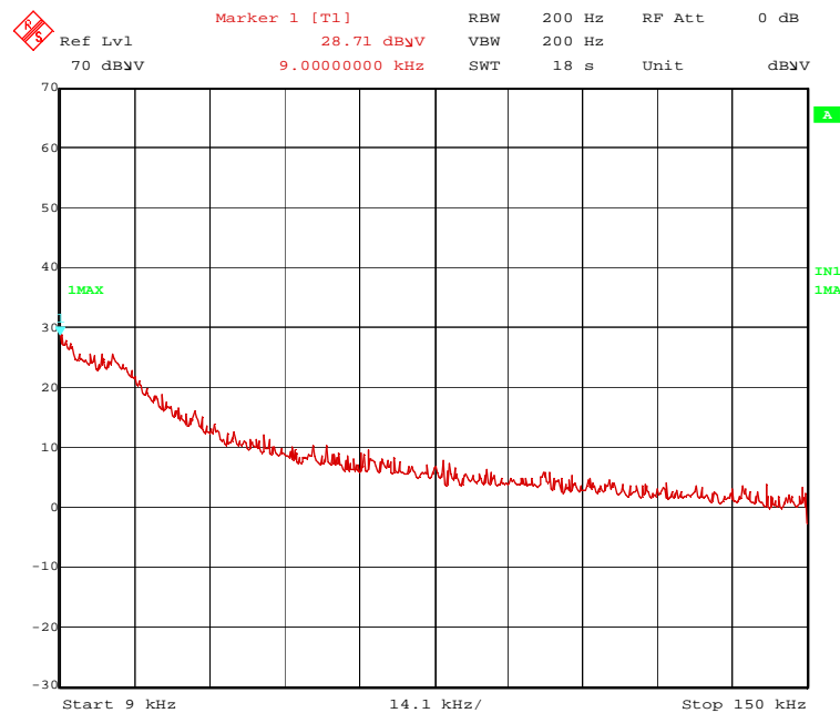
134118a.wmf: Spurious emissions from 9 kHz to 150 kHz
