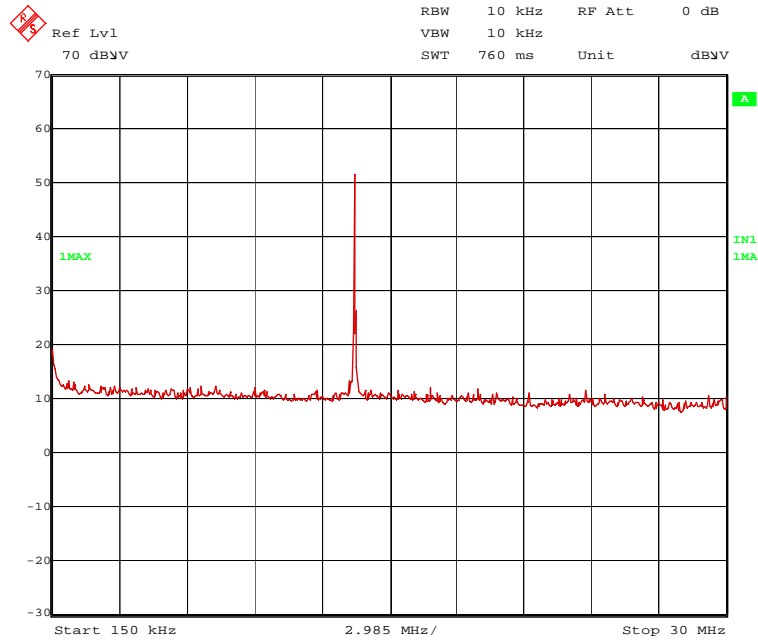
134117b.wmf: Spurious emissions from 150 kHz to 30 MHz
