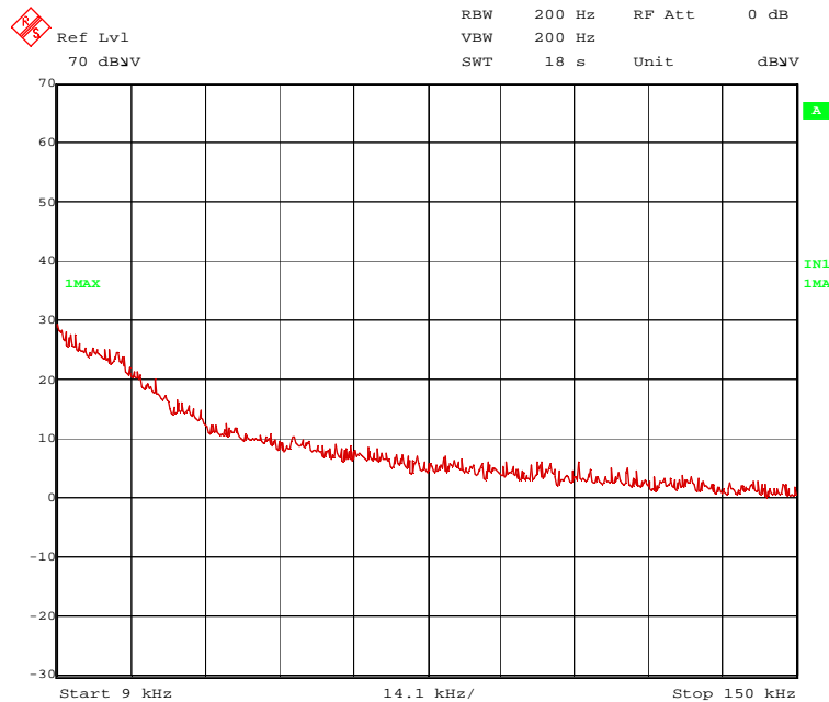
134117a.wmf: Spurious emissions from 9 kHz to 150 kHz
