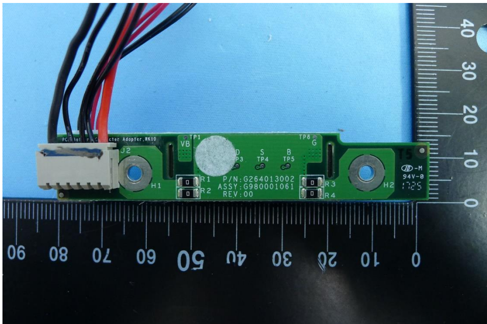
(29) EUT Photo
