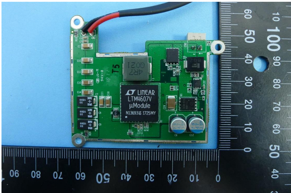
(27) EUT Photo
