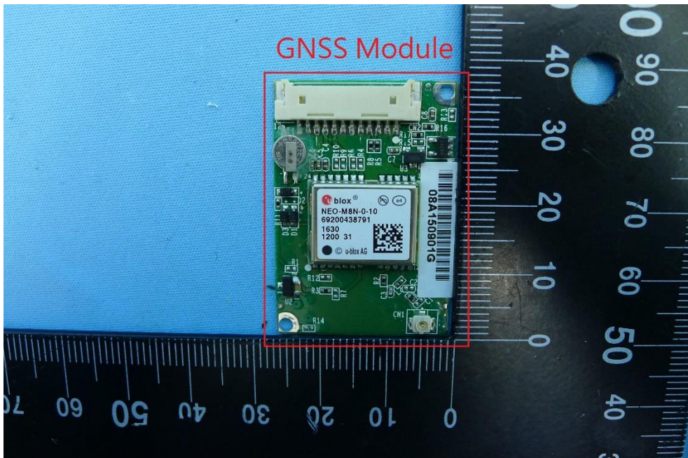
(35) EUT Photo
