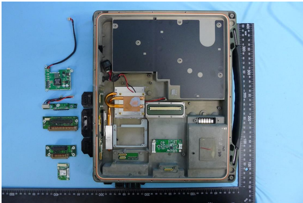
(27) EUT Photo
