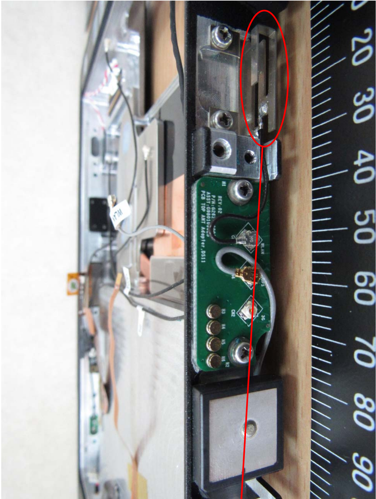
ANT A (2.4G_WLAN): PIFA antenna / 1.87 dBi ANT A (5G_WLAN): PIFA antenna / 4.74 dBi
